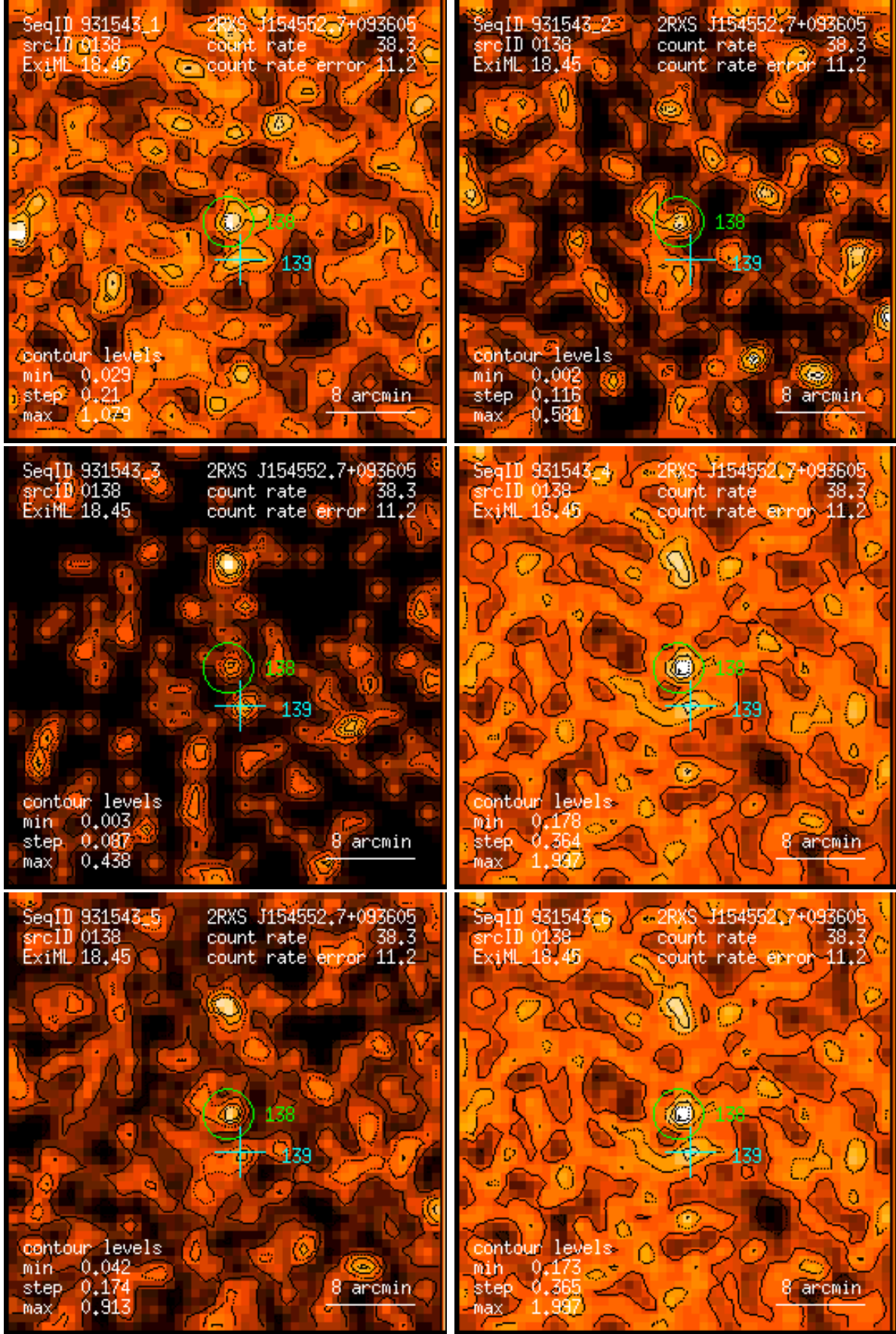
Figure 138: RASS 931543: detection 0138: band rate images, Gaussian filter: (1) PSPC channels 11 – 41, (2) 52 – 90, (3) 91 – 201, (4) 11 – 235, (5) 52 – 201, (6) 11 – 201. Broad band rates in counts/ks. Band rate contour levels in counts/ks/arcmin 2 .
