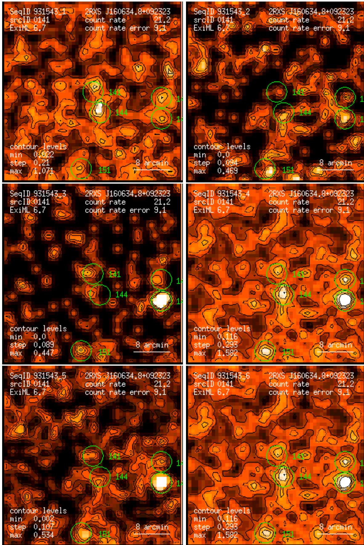
Figure 141: RASS 931543: detection 0141: band rate images, Gaussian filter: (1) PSPC channels 11 – 41, (2) 52 – 90, (3) 91 – 201, (4) 11 – 235, (5) 52 – 201, (6) 11 – 201. Broad band rates in counts/ks. Band rate contour levels in counts/ks/arcmin 2 .
