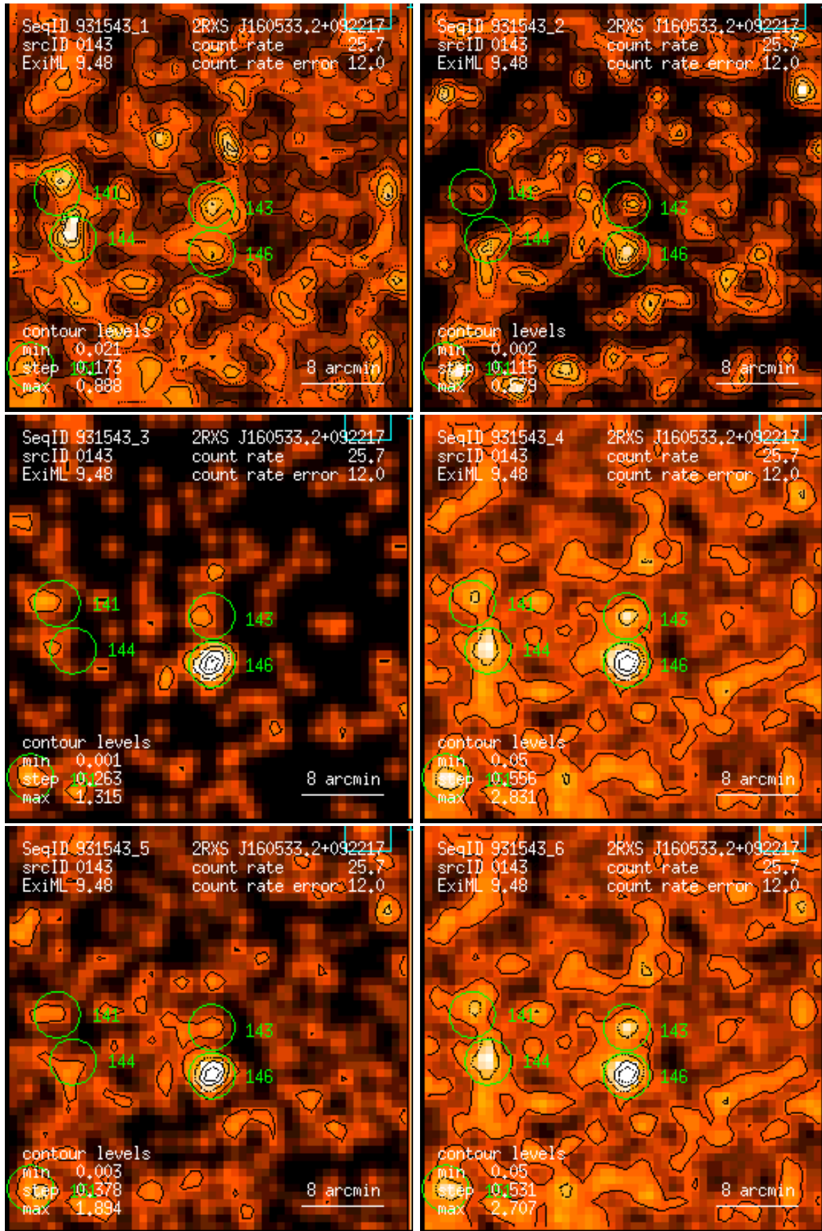
Figure 143: RASS 931543: detection 0143: band rate images, Gaussian filter: (1) PSPC channels 11 – 41, (2) 52 – 90, (3) 91 – 201, (4) 11 – 235, (5) 52 – 201, (6) 11 – 201. Broad band rates in counts/ks. Band rate contour levels in counts/ks/arcmin 2 .
