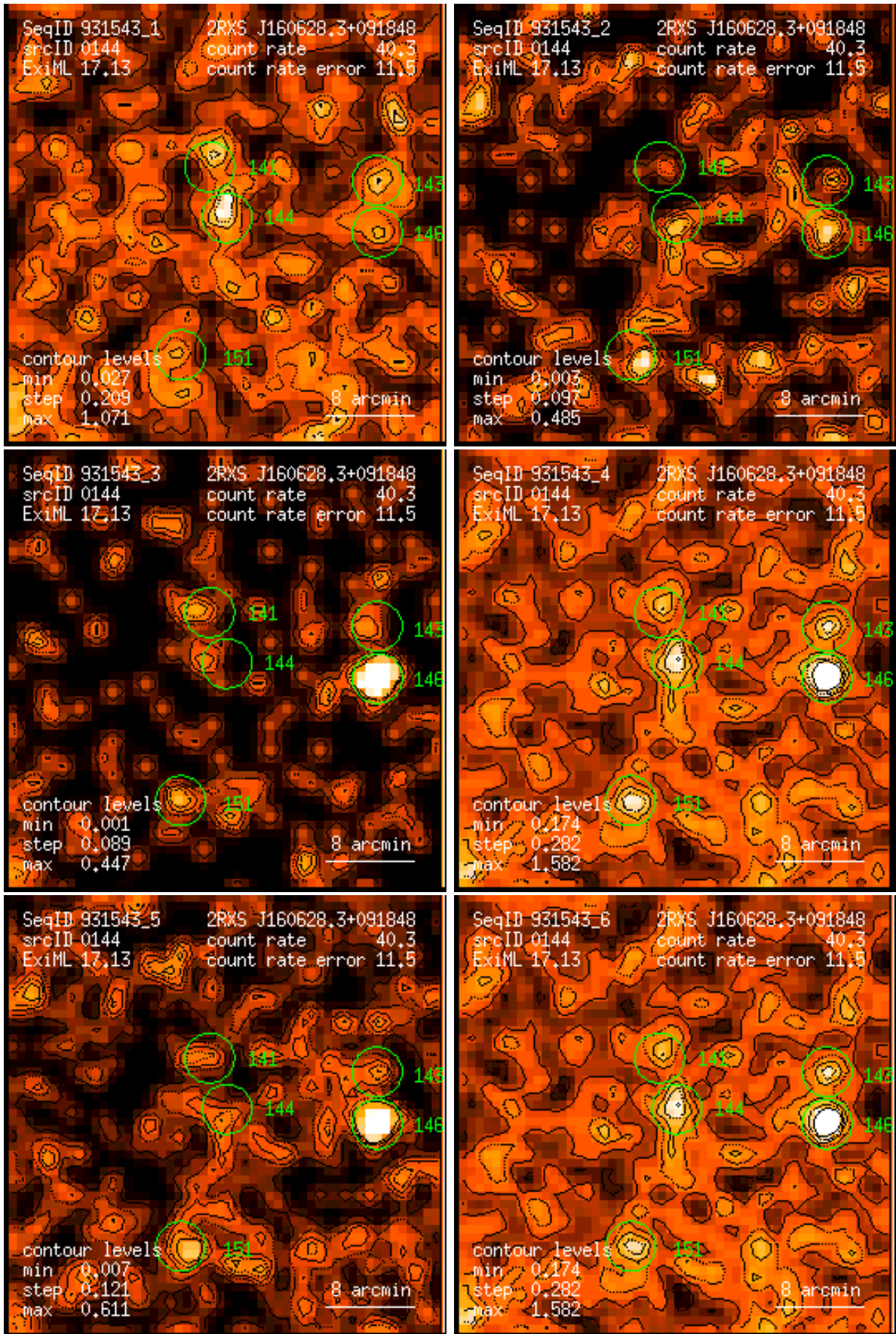
Figure 144: RASS 931543: detection 0144: band rate images, Gaussian filter: (1) PSPC channels 11 – 41, (2) 52 – 90, (3) 91 – 201, (4) 11 – 235, (5) 52 – 201, (6) 11 – 201. Broad band rates in counts/ks. Band rate contour levels in counts/ks/arcmin 2 .
