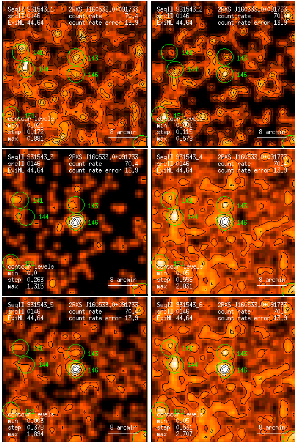
Figure 146: RASS 931543: detection 0146: band rate images, Gaussian filter: (1) PSPC channels 11 – 41, (2) 52 – 90, (3) 91 – 201, (4) 11 – 235, (5) 52 – 201, (6) 11 – 201. Broad band rates in counts/ks. Band rate contour levels in counts/ks/arcmin 2 .
