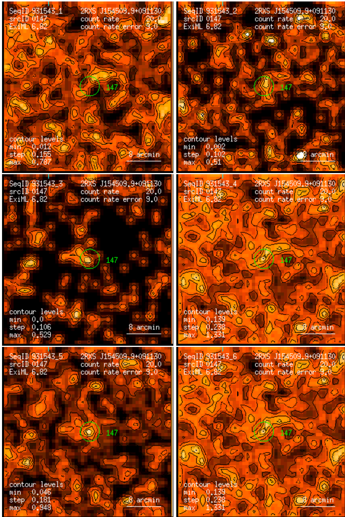
Figure 147: RASS 931543: detection 0147: band rate images, Gaussian filter: (1) PSPC channels 11 – 41, (2) 52 – 90, (3) 91 – 201, (4) 11 – 235, (5) 52 – 201, (6) 11 – 201. Broad band rates in counts/ks. Band rate contour levels in counts/ks/arcmin 2 .
