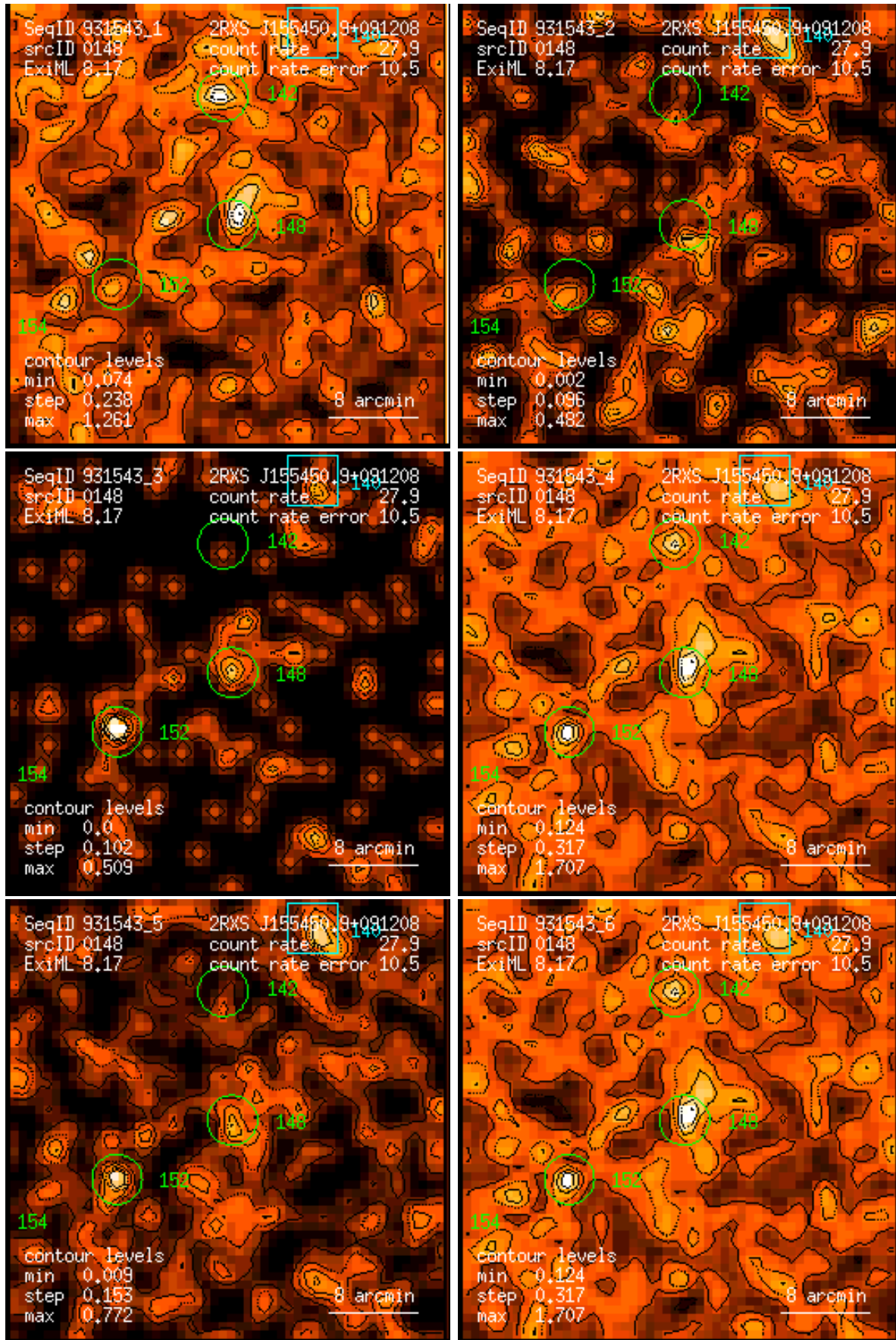
Figure 148: RASS 931543: detection 0148: band rate images, Gaussian filter: (1) PSPC channels 11 – 41, (2) 52 – 90, (3) 91 – 201, (4) 11 – 235, (5) 52 – 201, (6) 11 – 201. Broad band rates in counts/ks. Band rate contour levels in counts/ks/arcmin 2 .
