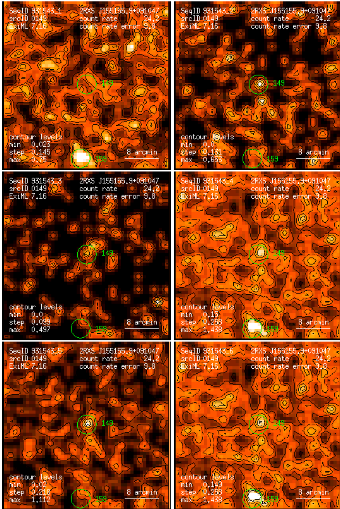
Figure 149: RASS 931543: detection 0149: band rate images, Gaussian filter: (1) PSPC channels 11 – 41, (2) 52 – 90, (3) 91 – 201, (4) 11 – 235, (5) 52 – 201, (6) 11 – 201. Broad band rates in counts/ks. Band rate contour levels in counts/ks/arcmin 2 .
