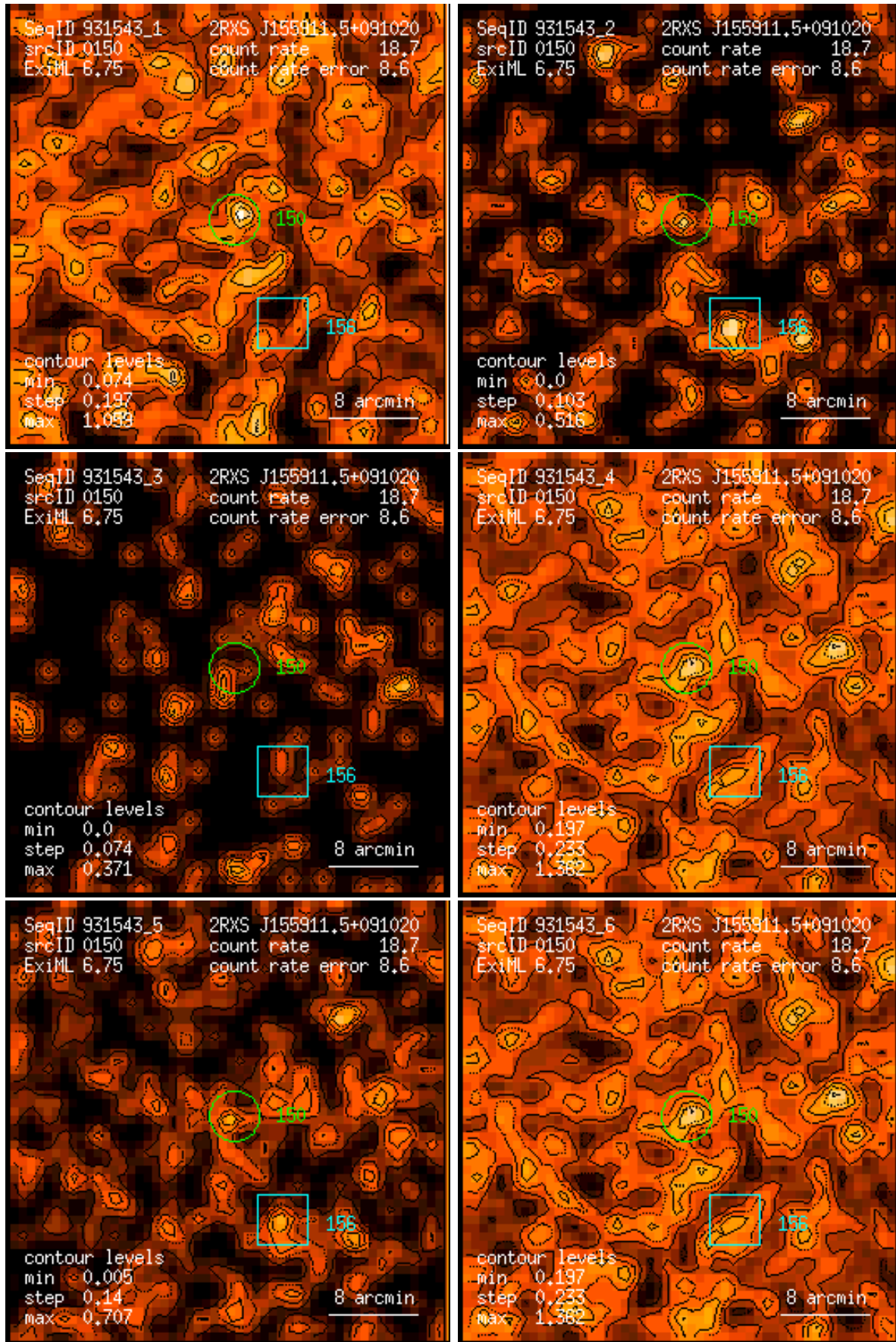
Figure 150: RASS 931543: detection 0150: band rate images, Gaussian filter: (1) PSPC channels 11 – 41, (2) 52 – 90, (3) 91 – 201, (4) 11 – 235, (5) 52 – 201, (6) 11 – 201. Broad band rates in counts/ks. Band rate contour levels in counts/ks/arcmin 2 .
