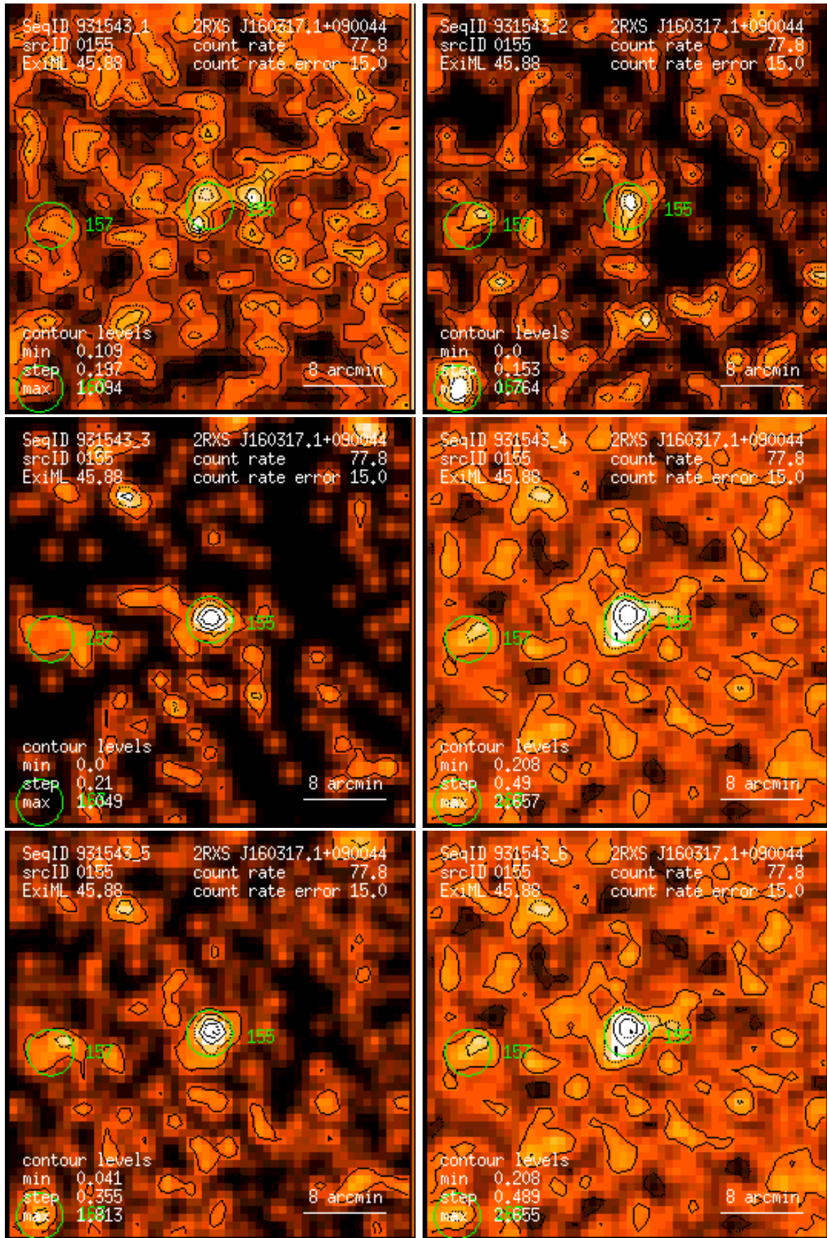
Figure 155: RASS 931543: detection 0155: band rate images, Gaussian filter: (1) PSPC channels 11 – 41, (2) 52 – 90, (3) 91 – 201, (4) 11 – 235, (5) 52 – 201, (6) 11 – 201. Broad band rates in counts/ks. Band rate contour levels in counts/ks/arcmin 2 .
