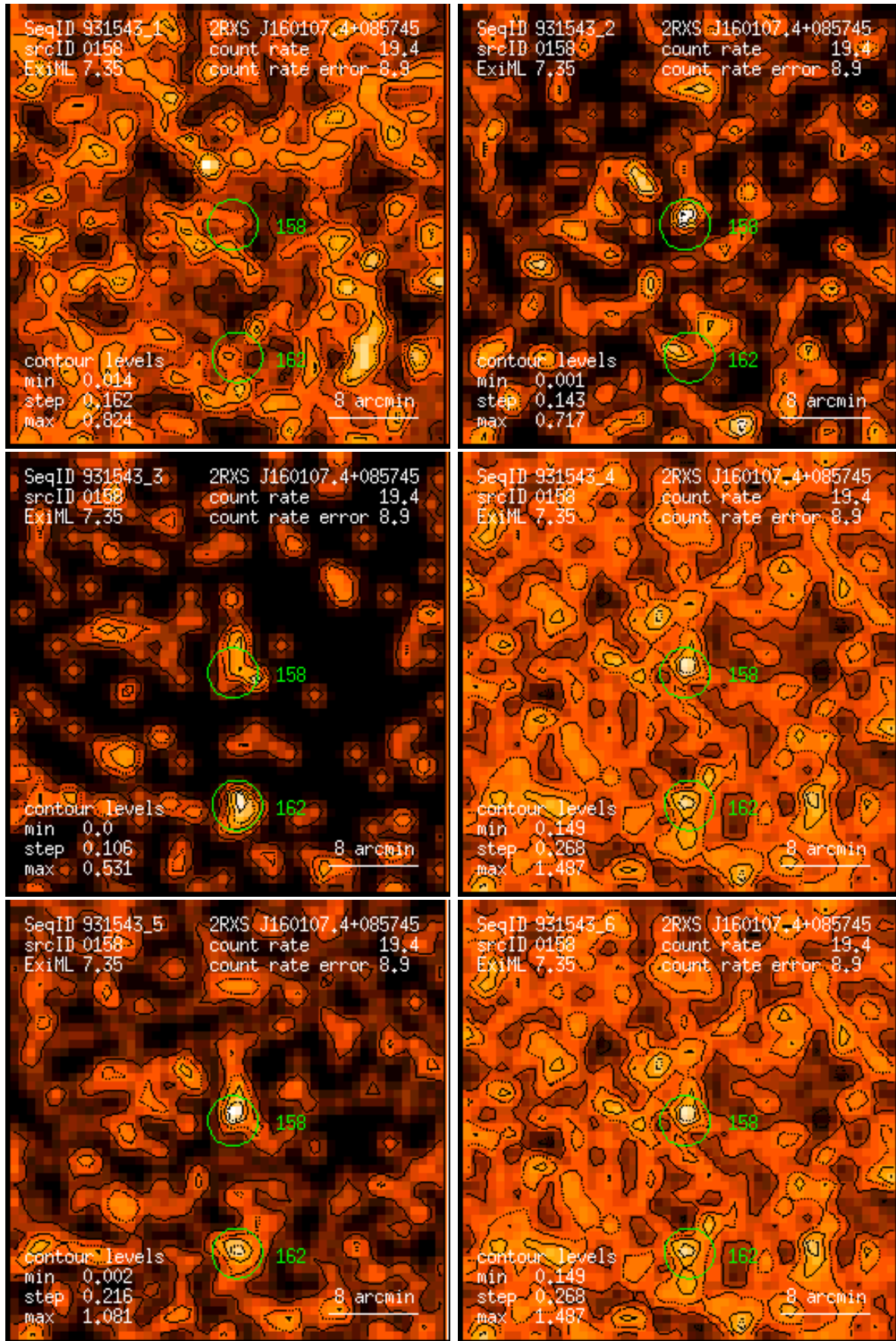
Figure 158: RASS 931543: detection 0158: band rate images, Gaussian filter: (1) PSPC channels 11 – 41, (2) 52 – 90, (3) 91 – 201, (4) 11 – 235, (5) 52 – 201, (6) 11 – 201. Broad band rates in counts/ks. Band rate contour levels in counts/ks/arcmin 2 .
