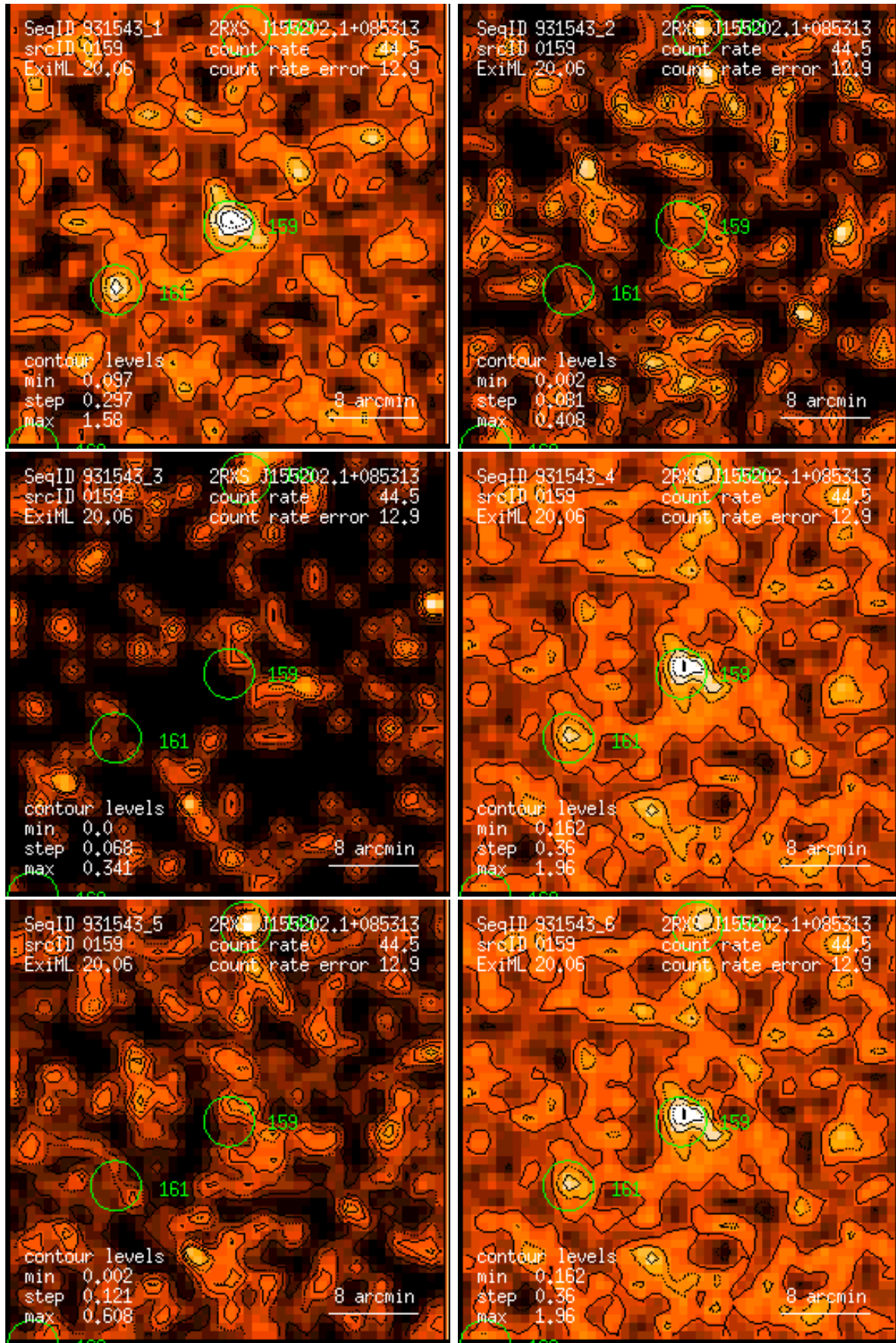
Figure 159: RASS 931543: detection 0159: band rate images, Gaussian filter: (1) PSPC channels 11 – 41, (2) 52 – 90, (3) 91 – 201, (4) 11 – 235, (5) 52 – 201, (6) 11 – 201. Broad band rates in counts/ks. Band rate contour levels in counts/ks/arcmin 2 .
