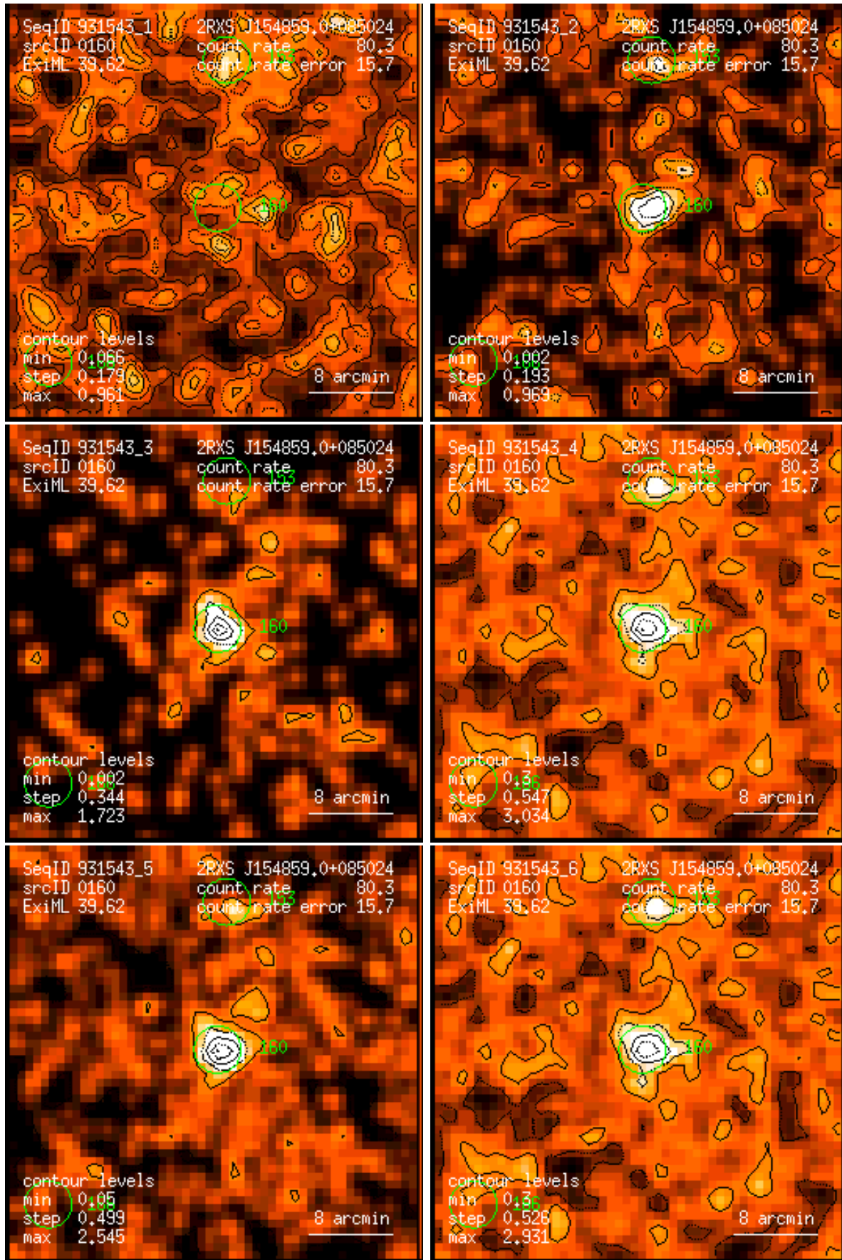
Figure 160: RASS 931543: detection 0160: band rate images, Gaussian filter: (1) PSPC channels 11 – 41, (2) 52 – 90, (3) 91 – 201, (4) 11 – 235, (5) 52 – 201, (6) 11 – 201. Broad band rates in counts/ks. Band rate contour levels in counts/ks/arcmin 2 .
