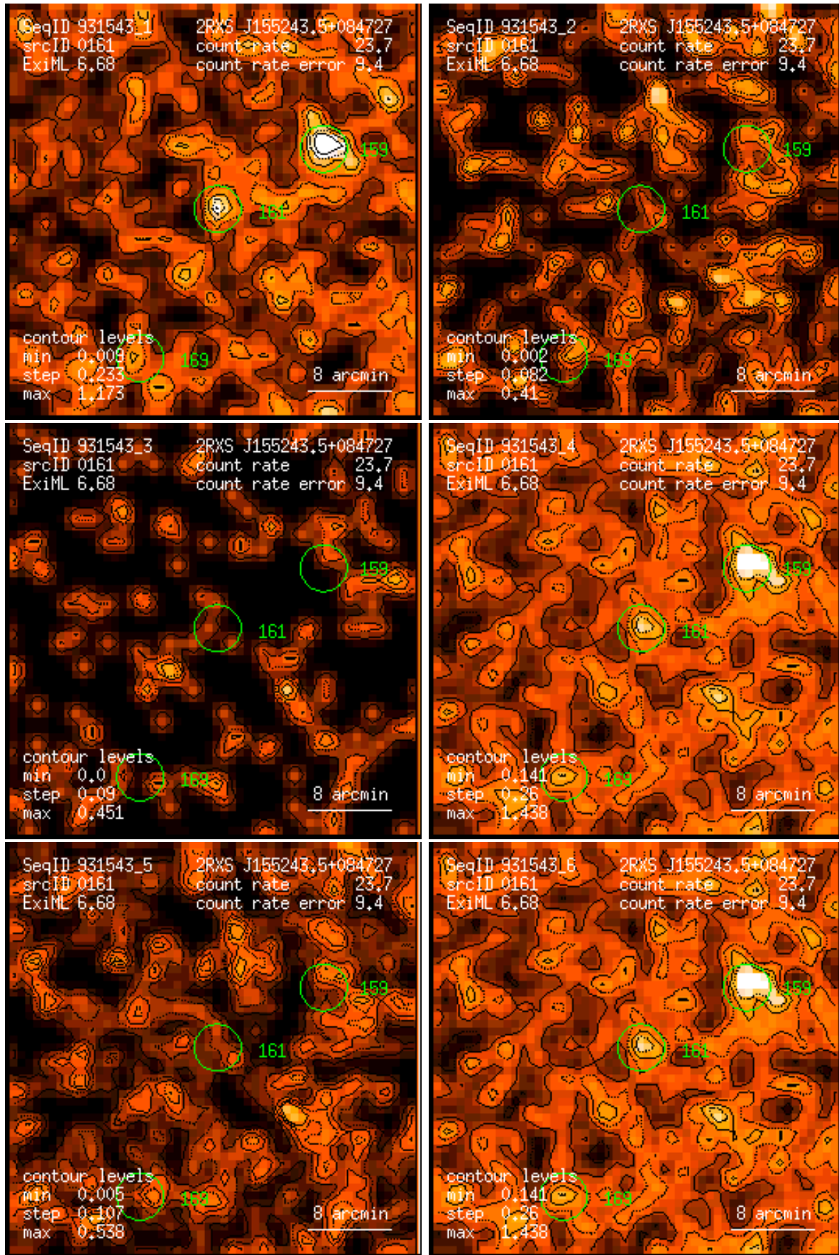
Figure 161: RASS 931543: detection 0161: band rate images, Gaussian filter: (1) PSPC channels 11 – 41, (2) 52 – 90, (3) 91 – 201, (4) 11 – 235, (5) 52 – 201, (6) 11 – 201. Broad band rates in counts/ks. Band rate contour levels in counts/ks/arcmin 2 .
