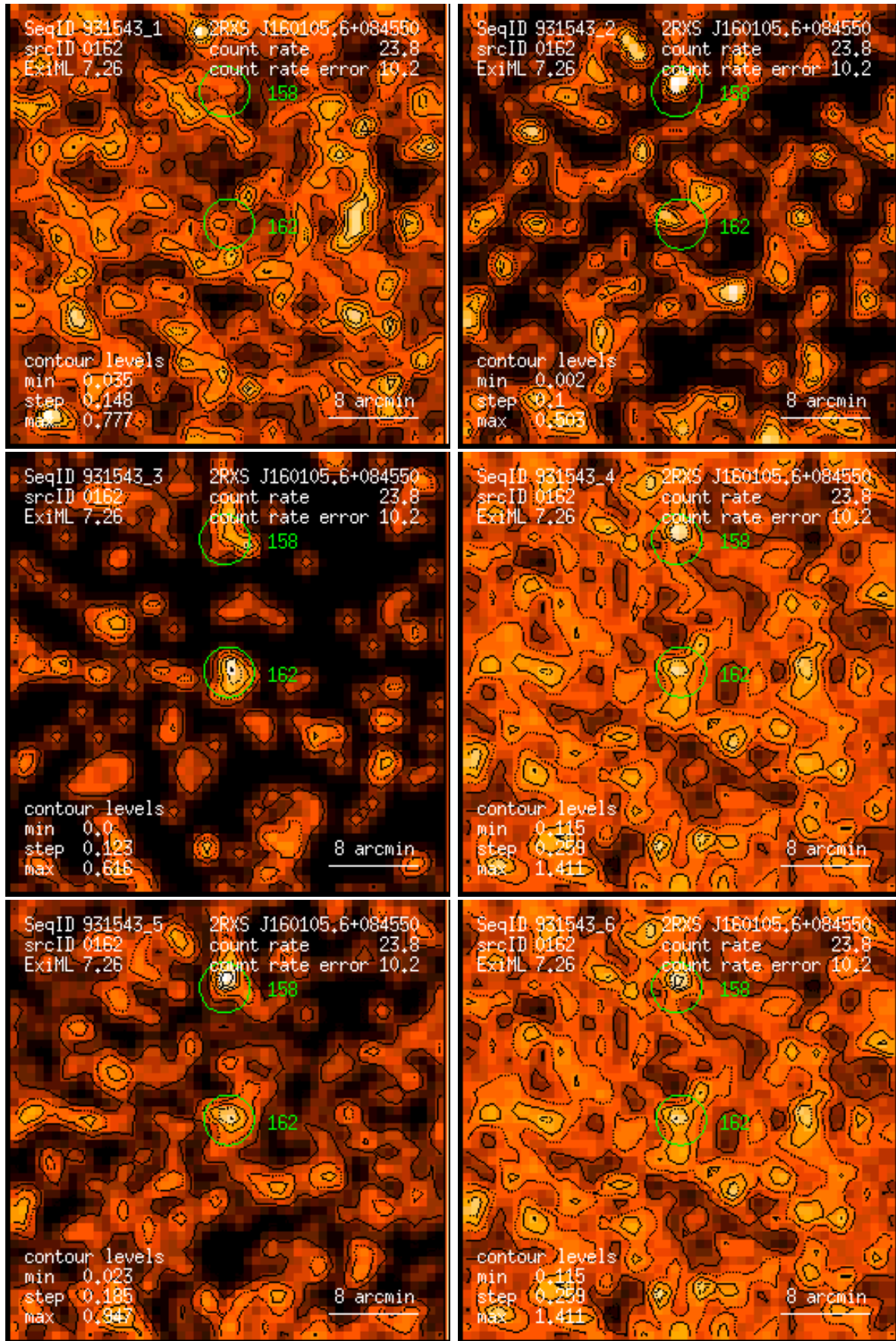
Figure 162: RASS 931543: detection 0162: band rate images, Gaussian filter: (1) PSPC channels 11 – 41, (2) 52 – 90, (3) 91 – 201, (4) 11 – 235, (5) 52 – 201, (6) 11 – 201. Broad band rates in counts/ks. Band rate contour levels in counts/ks/arcmin 2 .
