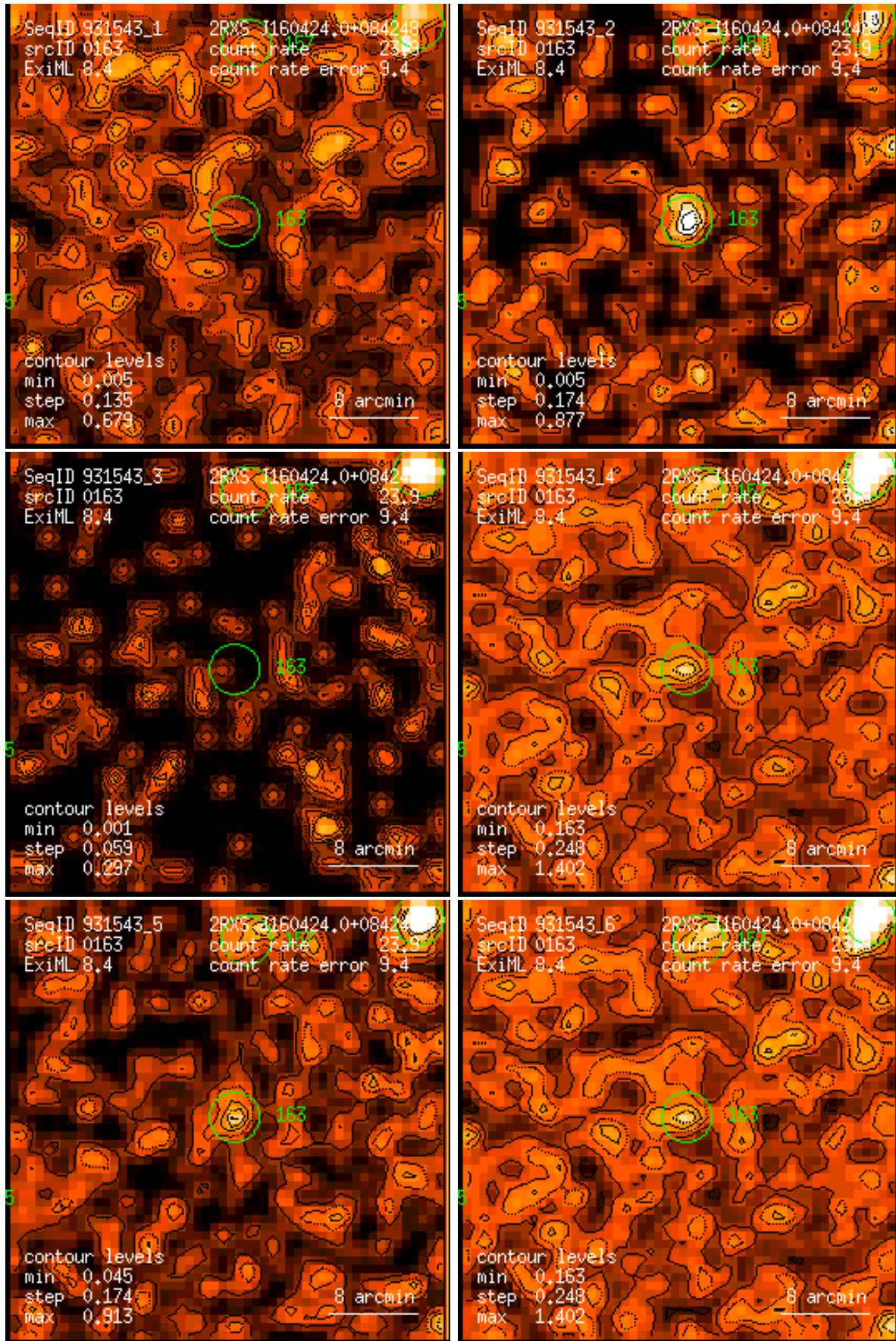
Figure 163: RASS 931543: detection 0163: band rate images, Gaussian filter: (1) PSPC channels 11 – 41, (2) 52 – 90, (3) 91 – 201, (4) 11 – 235, (5) 52 – 201, (6) 11 – 201. Broad band rates in counts/ks. Band rate contour levels in counts/ks/arcmin 2 .
