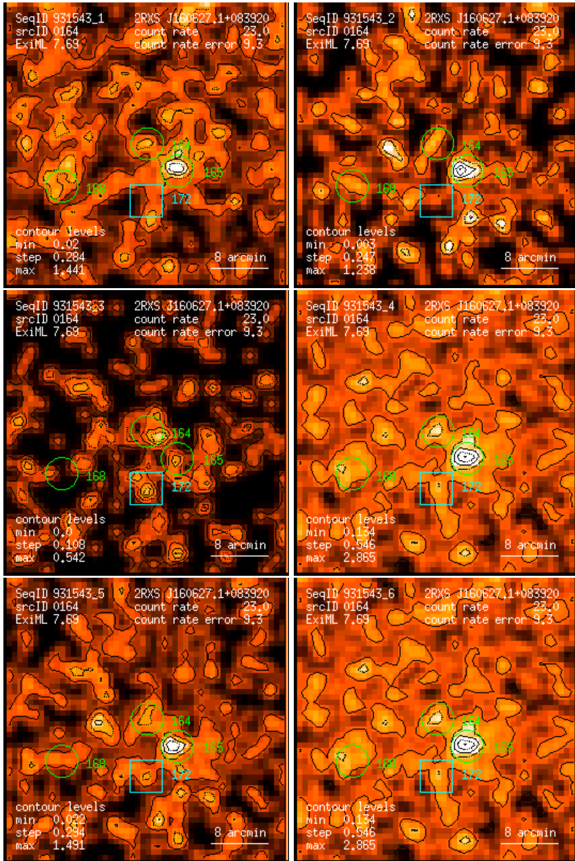
Figure 164: RASS 931543: detection 0164: band rate images, Gaussian filter: (1) PSPC channels 11 – 41, (2) 52 – 90, (3) 91 – 201, (4) 11 – 235, (5) 52 – 201, (6) 11 – 201. Broad band rates in counts/ks. Band rate contour levels in counts/ks/arcmin 2 .
