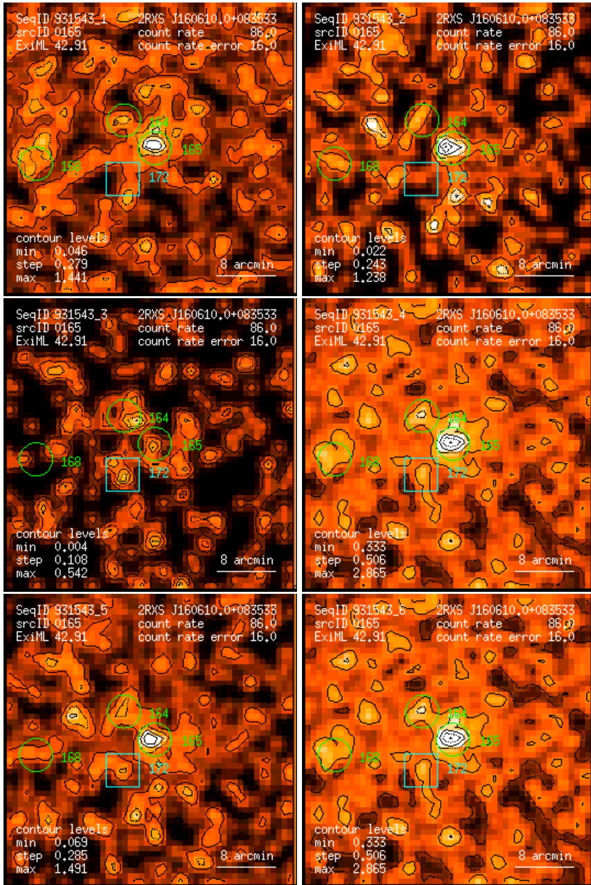
Figure 165: RASS 931543: detection 0165: band rate images, Gaussian filter: (1) PSPC channels 11 – 41, (2) 52 – 90, (3) 91 – 201, (4) 11 – 235, (5) 52 – 201, (6) 11 – 201. Broad band rates in counts/ks. Band rate contour levels in counts/ks/arcmin 2 .
