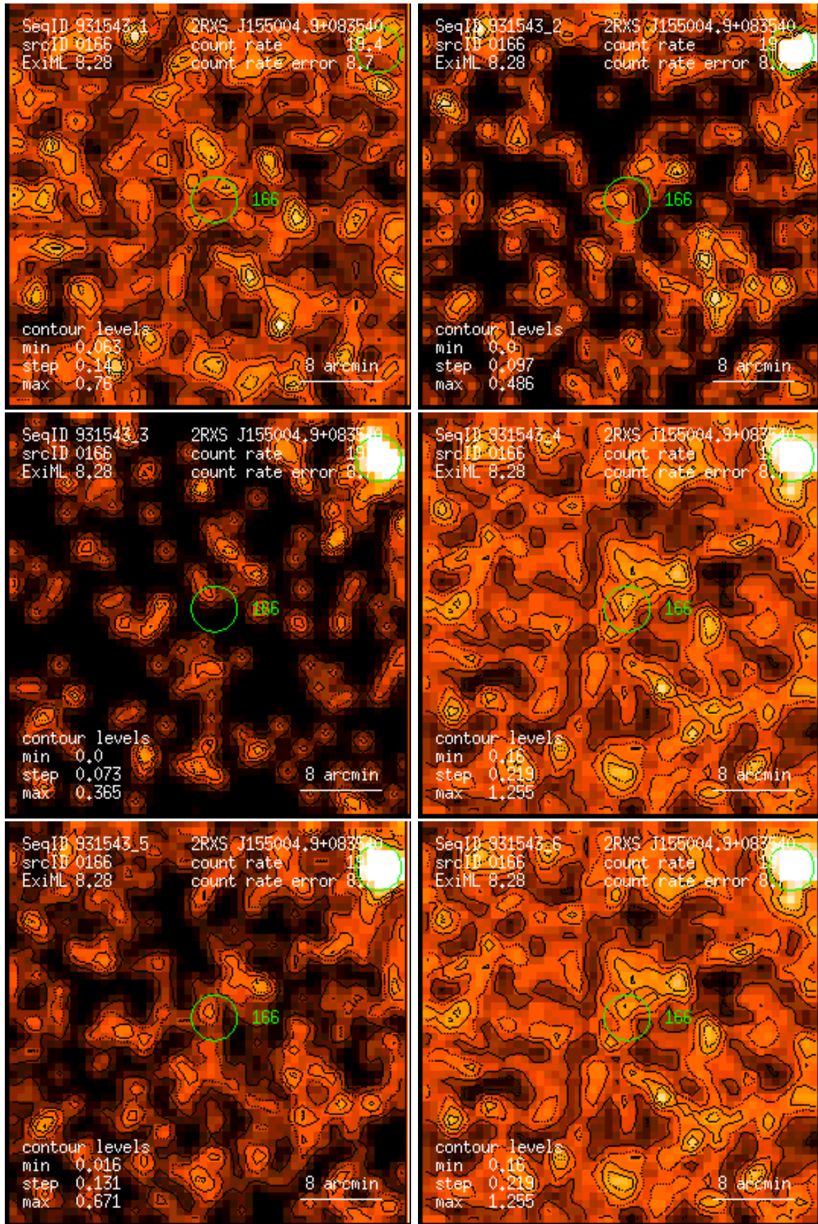
Figure 166: RASS 931543: detection 0166: band rate images, Gaussian filter: (1) PSPC channels 11 – 41, (2) 52 – 90, (3) 91 – 201, (4) 11 – 235, (5) 52 – 201, (6) 11 – 201. Broad band rates in counts/ks. Band rate contour levels in counts/ks/arcmin 2 .
