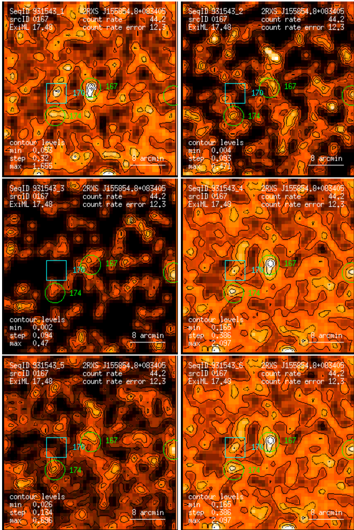
Figure 167: RASS 931543: detection 0167: band rate images, Gaussian filter: (1) PSPC channels 11 – 41, (2) 52 – 90, (3) 91 – 201, (4) 11 – 235, (5) 52 – 201, (6) 11 – 201. Broad band rates in counts/ks. Band rate contour levels in counts/ks/arcmin 2 .
