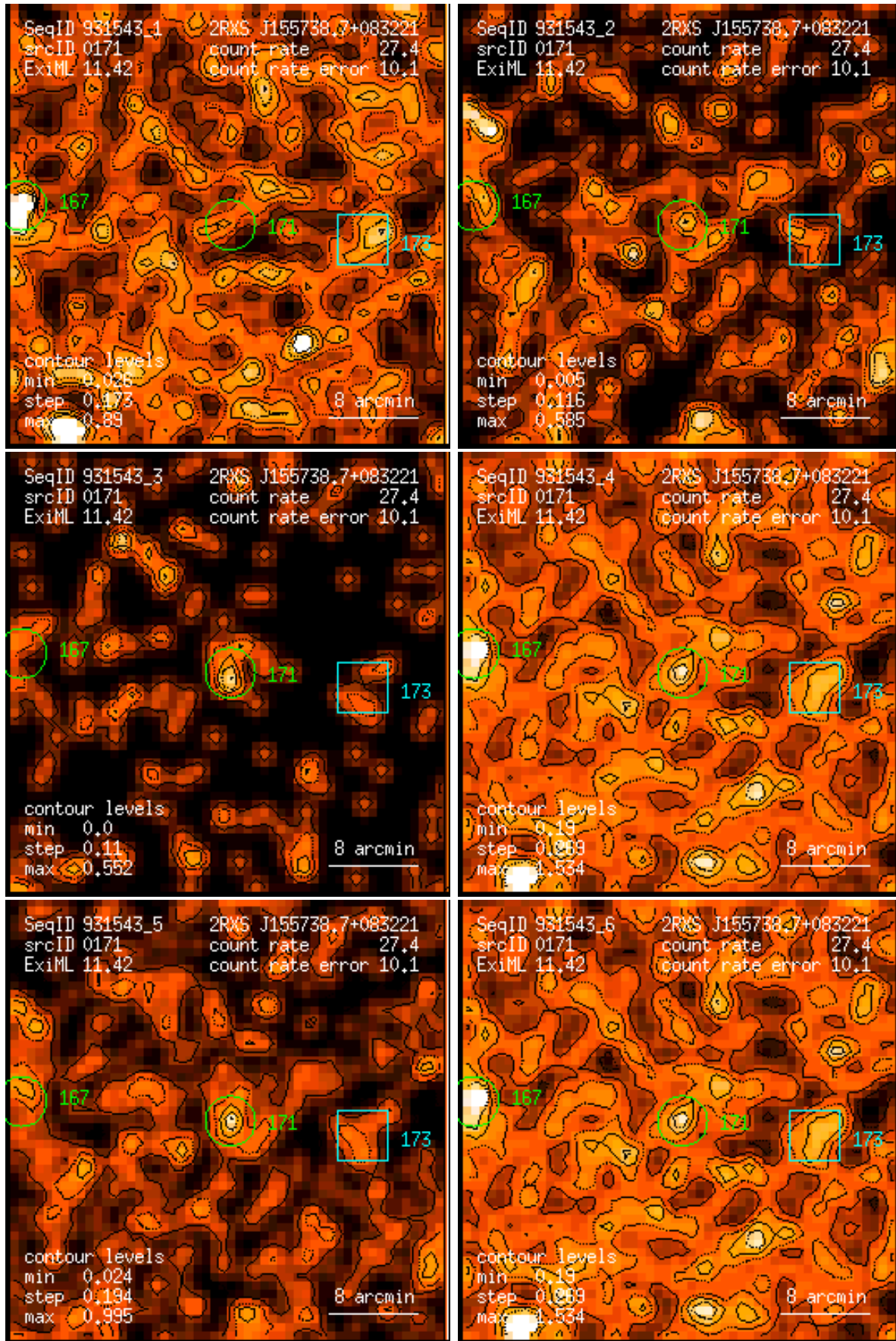
Figure 171: RASS 931543: detection 0171: band rate images, Gaussian filter: (1) PSPC channels 11 – 41, (2) 52 – 90, (3) 91 – 201, (4) 11 – 235, (5) 52 – 201, (6) 11 – 201. Broad band rates in counts/ks. Band rate contour levels in counts/ks/arcmin 2 .
