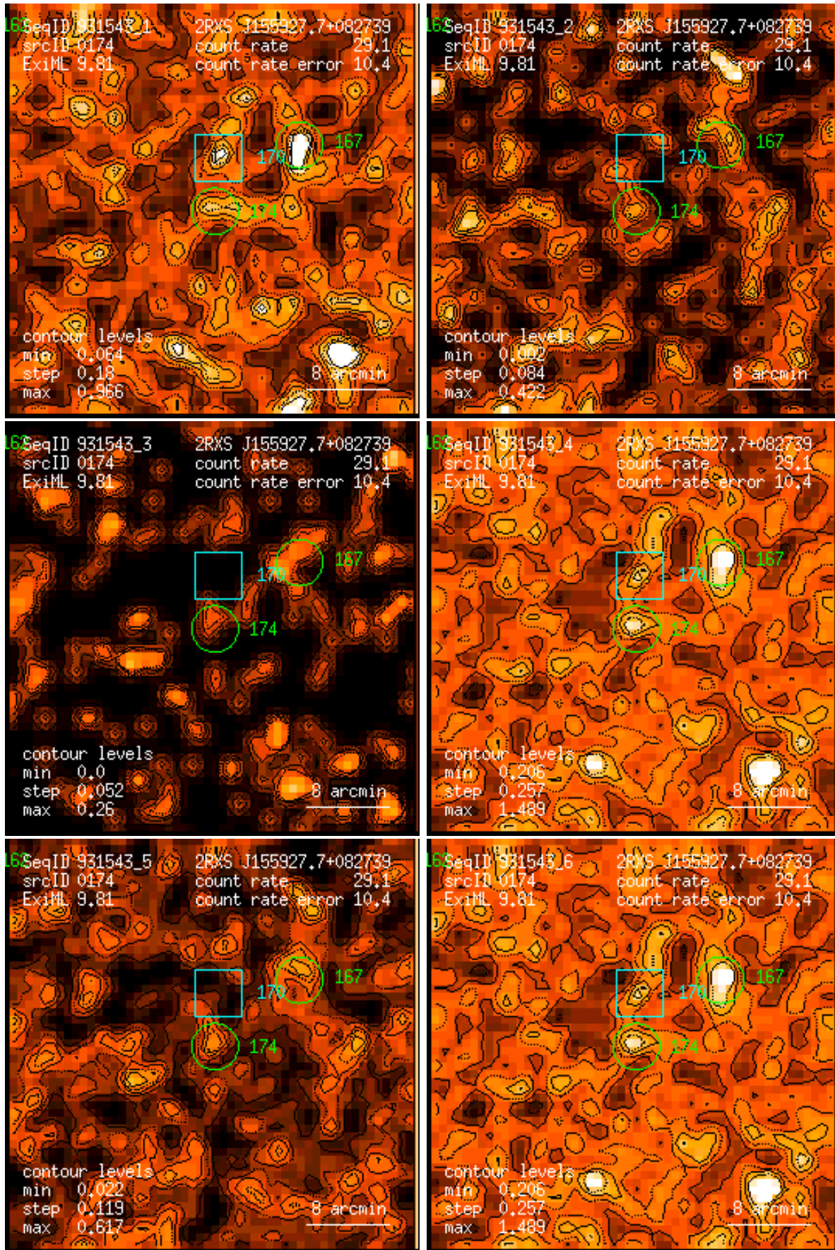
Figure 174: RASS 931543: detection 0174: band rate images, Gaussian filter: (1) PSPC channels 11 – 41, (2) 52 – 90, (3) 91 – 201, (4) 11 – 235, (5) 52 – 201, (6) 11 – 201. Broad band rates in counts/ks. Band rate contour levels in counts/ks/arcmin 2 .
