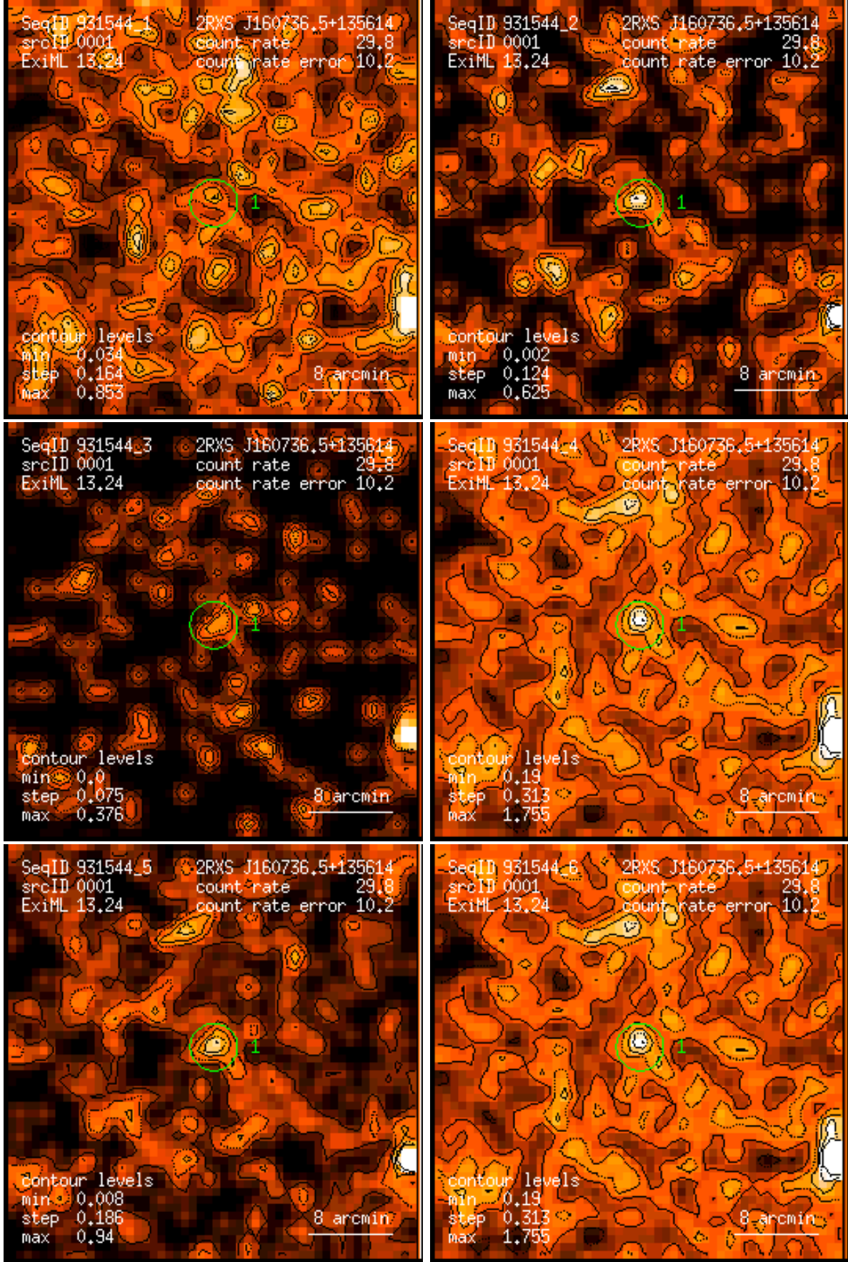
Figure 1: RASS 931544: detection 0001: band rate images, Gaussian filter: (1) PSPC channels 11 – 41, (2) 52 – 90, (3) 91 – 201, (4) 11 – 235, (5) 52 – 201, (6) 11 – 201. Broad band rates in counts/ks. Band rate contour levels in counts/ks/arcmin 2 .
