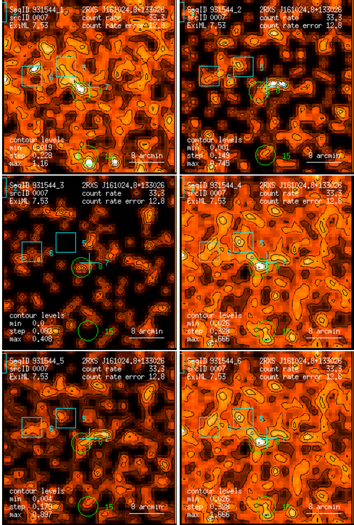
Figure 7: RASS 931544: detection 0007: band rate images, Gaussian filter: (1) PSPC channels 11 – 41, (2) 52 – 90, (3) 91 – 201, (4) 11 – 235, (5) 52 – 201, (6) 11 – 201. Broad band rates in counts/ks. Band rate contour levels in counts/ks/arcmin 2 .
