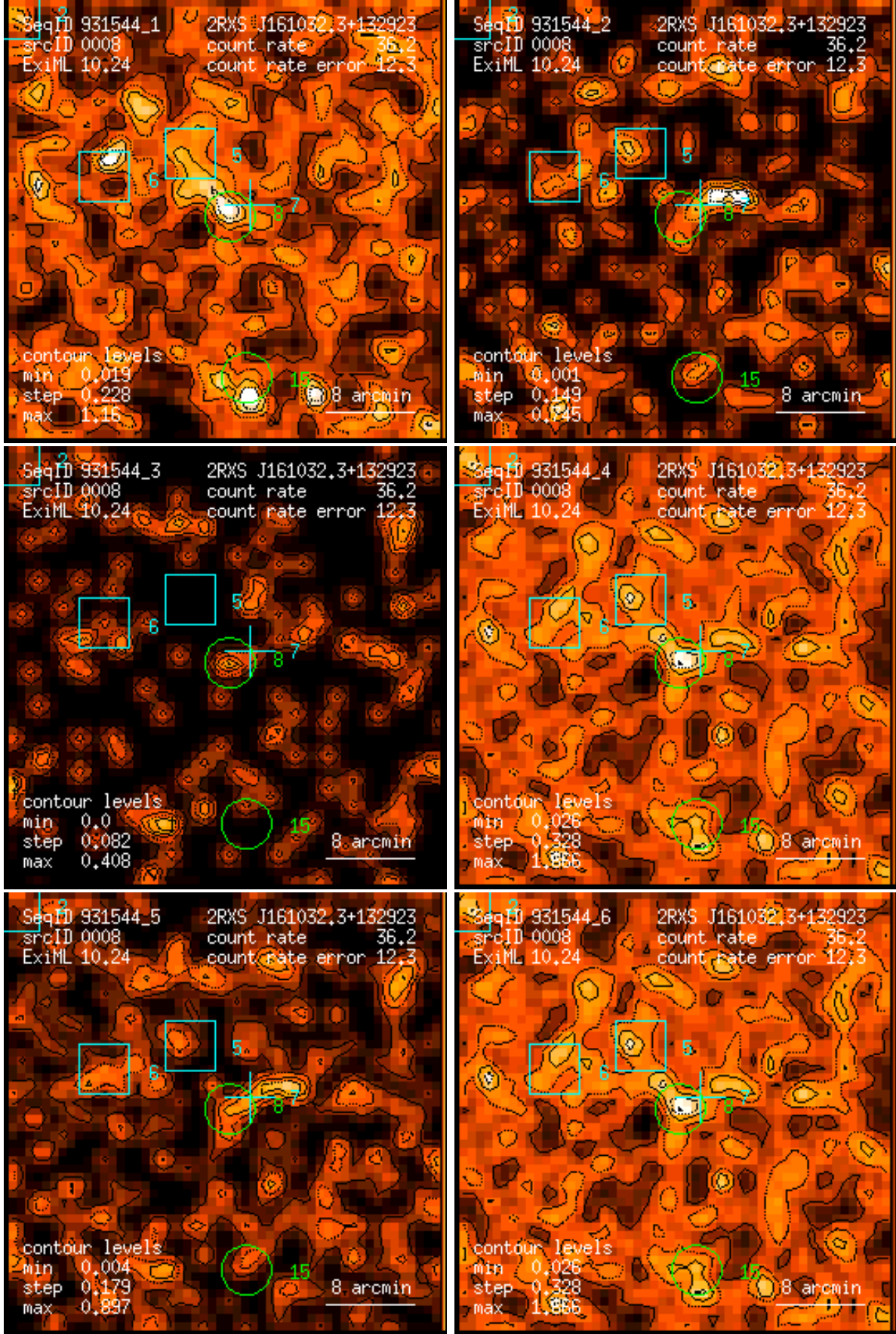
Figure 8: RASS 931544: detection 0008: band rate images, Gaussian filter: (1) PSPC channels 11 – 41, (2) 52 – 90, (3) 91 – 201, (4) 11 – 235, (5) 52 – 201, (6) 11 – 201. Broad band rates in counts/ks. Band rate contour levels in counts/ks/arcmin 2 .
