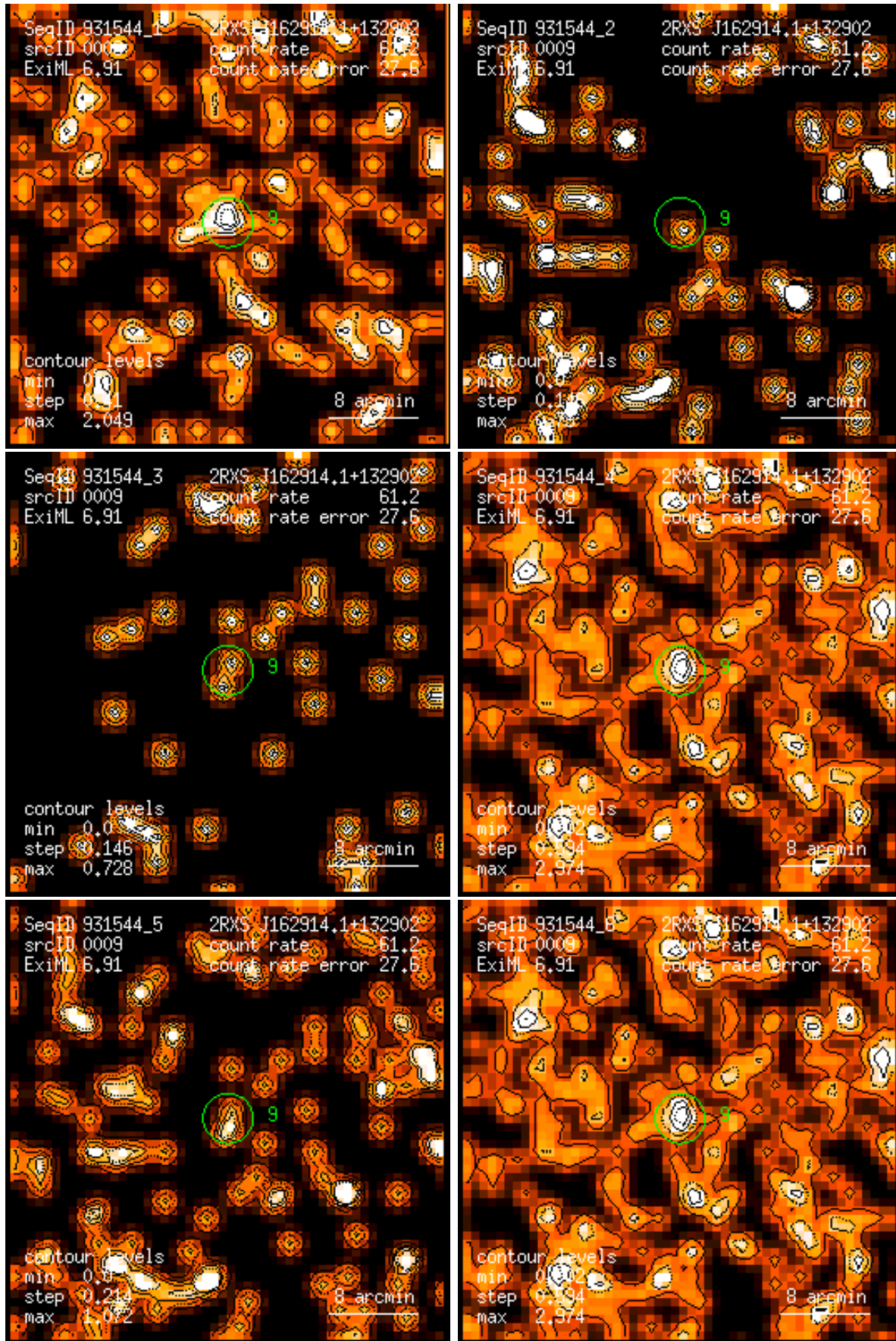
Figure 9: RASS 931544: detection 0009: band rate images, Gaussian filter: (1) PSPC channels 11 – 41, (2) 52 – 90, (3) 91 – 201, (4) 11 – 235, (5) 52 – 201, (6) 11 – 201. Broad band rates in counts/ks. Band rate contour levels in counts/ks/arcmin 2 .
