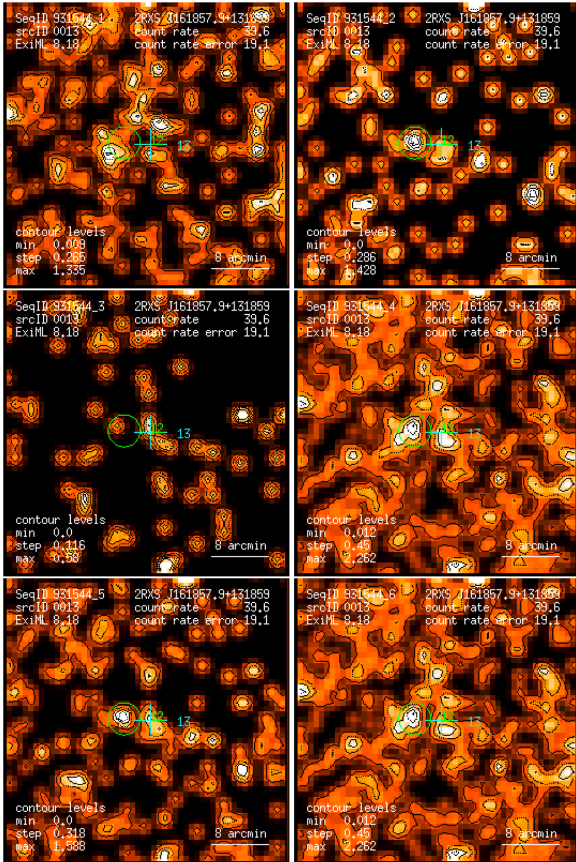
Figure 13: RASS 931544: detection 0013: band rate images, Gaussian filter: (1) PSPC channels 11 – 41, (2) 52 – 90, (3) 91 – 201, (4) 11 – 235, (5) 52 – 201, (6) 11 – 201. Broad band rates in counts/ks. Band rate contour levels in counts/ks/arcmin 2 .
