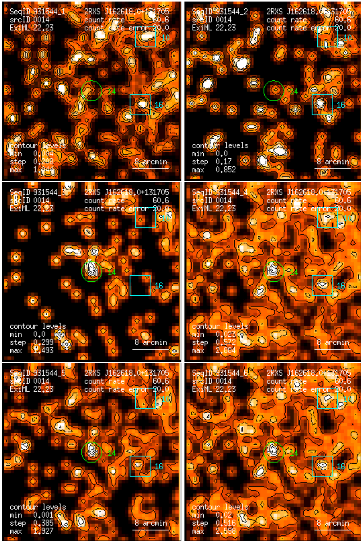
Figure 14: RASS 931544: detection 0014: band rate images, Gaussian filter: (1) PSPC channels 11 – 41, (2) 52 – 90, (3) 91 – 201, (4) 11 – 235, (5) 52 – 201, (6) 11 – 201. Broad band rates in counts/ks. Band rate contour levels in counts/ks/arcmin 2 .
