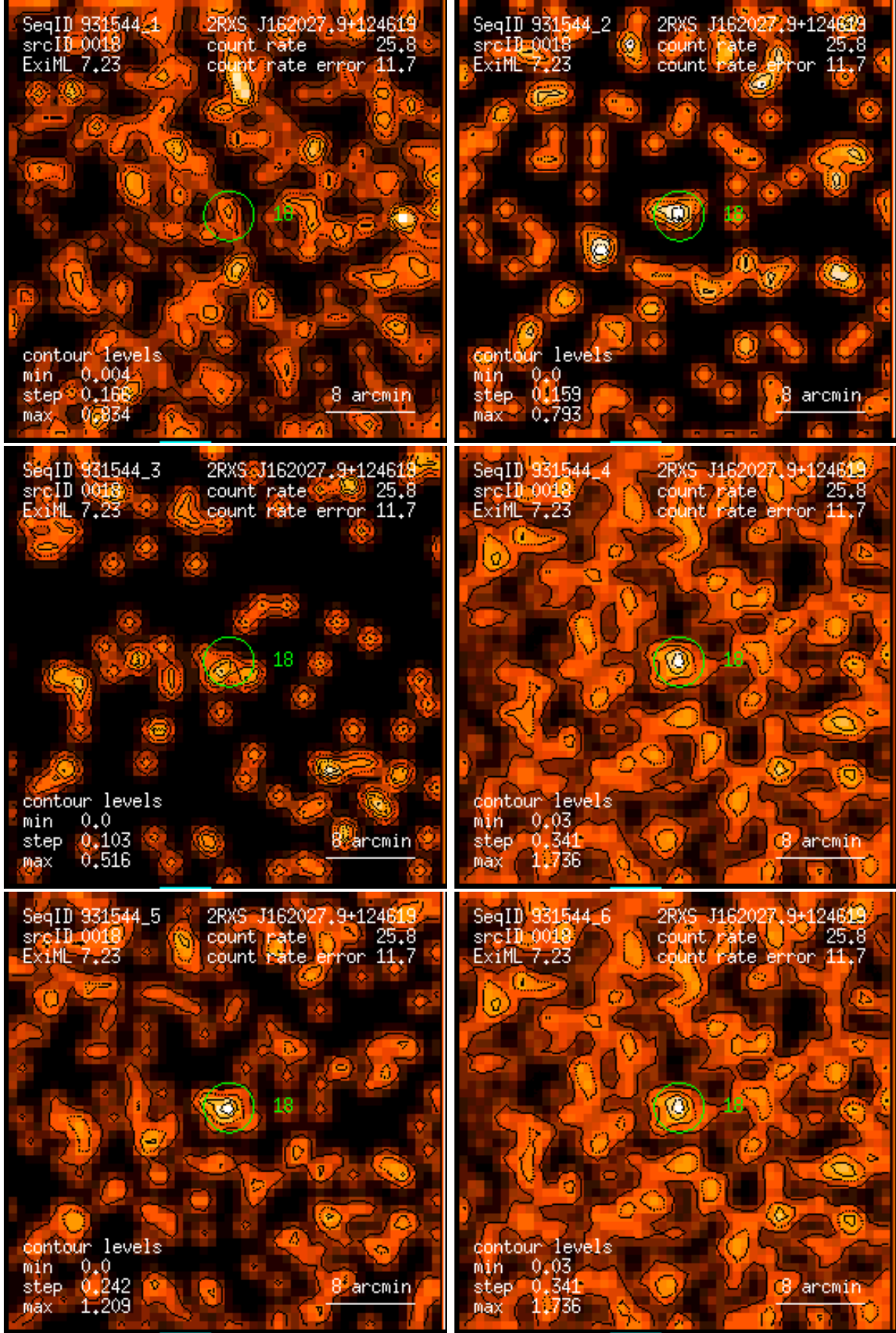
Figure 18: RASS 931544: detection 0018: band rate images, Gaussian filter: (1) PSPC channels 11 – 41, (2) 52 – 90, (3) 91 – 201, (4) 11 – 235, (5) 52 – 201, (6) 11 – 201. Broad band rates in counts/ks. Band rate contour levels in counts/ks/arcmin 2 .
