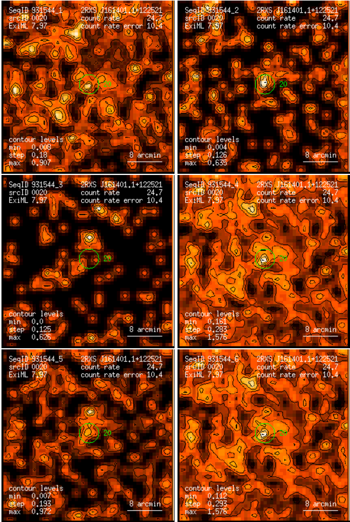
Figure 20: RASS 931544: detection 0020: band rate images, Gaussian filter: (1) PSPC channels 11 – 41, (2) 52 – 90, (3) 91 – 201, (4) 11 – 235, (5) 52 – 201, (6) 11 – 201. Broad band rates in counts/ks. Band rate contour levels in counts/ks/arcmin 2 .
