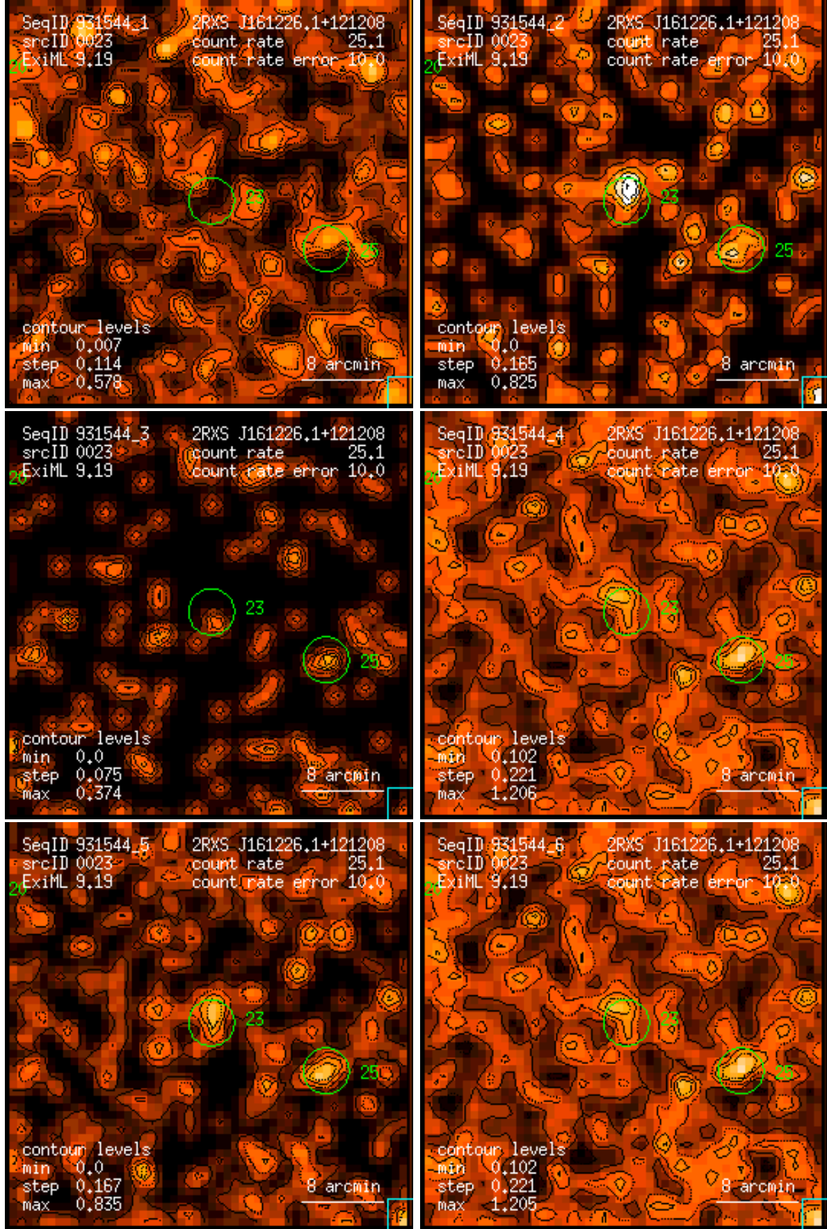
Figure 23: RASS 931544: detection 0023: band rate images, Gaussian filter: (1) PSPC channels 11 – 41, (2) 52 – 90, (3) 91 – 201, (4) 11 – 235, (5) 52 – 201, (6) 11 – 201. Broad band rates in counts/ks. Band rate contour levels in counts/ks/arcmin 2 .
