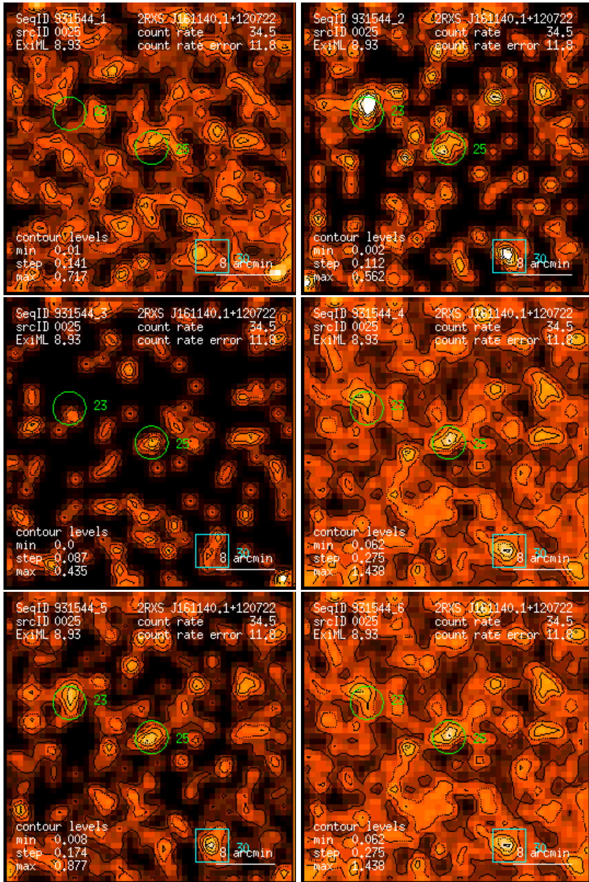
Figure 25: RASS 931544: detection 0025: band rate images, Gaussian filter: (1) PSPC channels 11 – 41, (2) 52 – 90, (3) 91 – 201, (4) 11 – 235, (5) 52 – 201, (6) 11 – 201. Broad band rates in counts/ks. Band rate contour levels in counts/ks/arcmin 2 .
