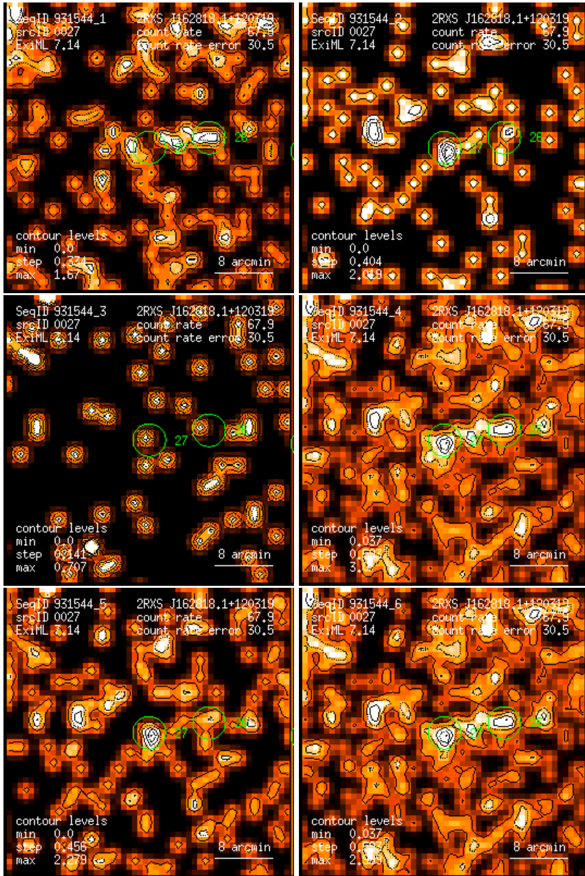
Figure 27: RASS 931544: detection 0027: band rate images, Gaussian filter: (1) PSPC channels 11 – 41, (2) 52 – 90, (3) 91 – 201, (4) 11 – 235, (5) 52 – 201, (6) 11 – 201. Broad band rates in counts/ks. Band rate contour levels in counts/ks/arcmin 2 .
