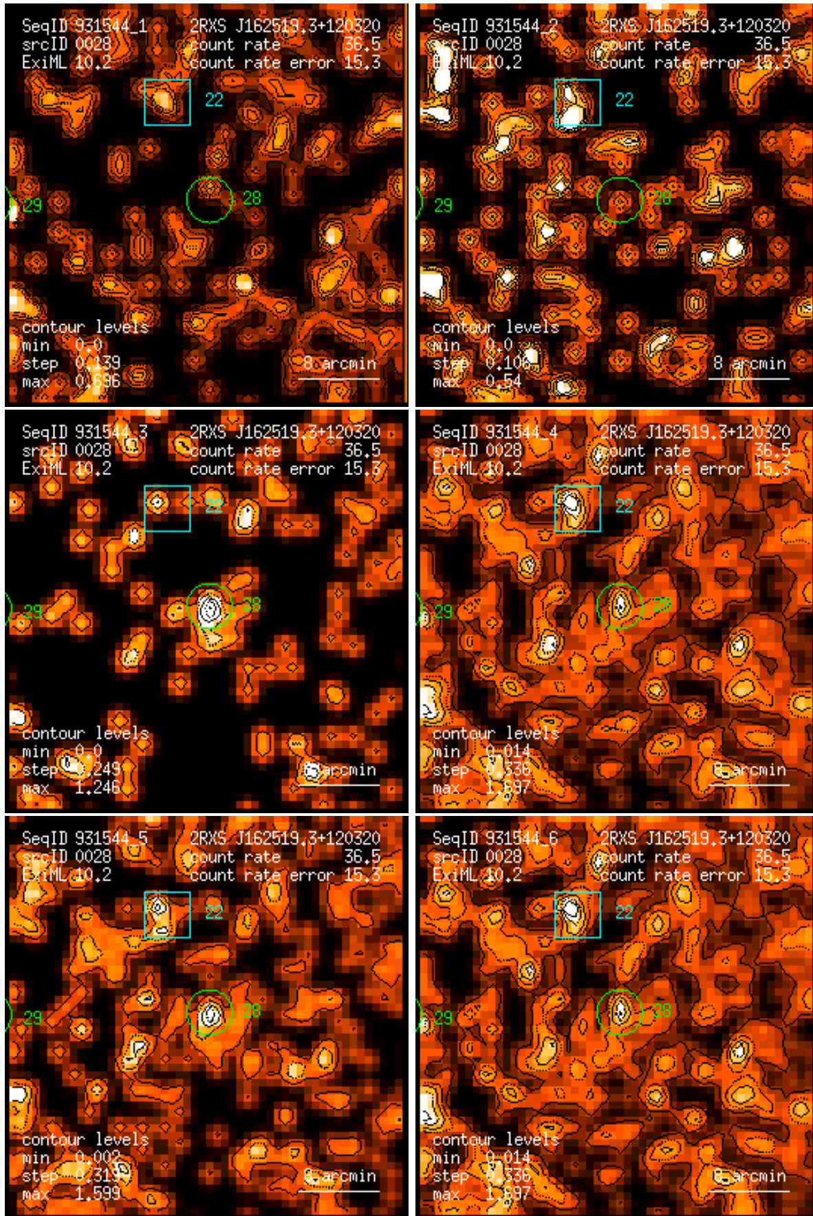
Figure 28: RASS 931544: detection 0028: band rate images, Gaussian filter: (1) PSPC channels 11 – 41, (2) 52 – 90, (3) 91 – 201, (4) 11 – 235, (5) 52 – 201, (6) 11 – 201. Broad band rates in counts/ks. Band rate contour levels in counts/ks/arcmin 2 .
