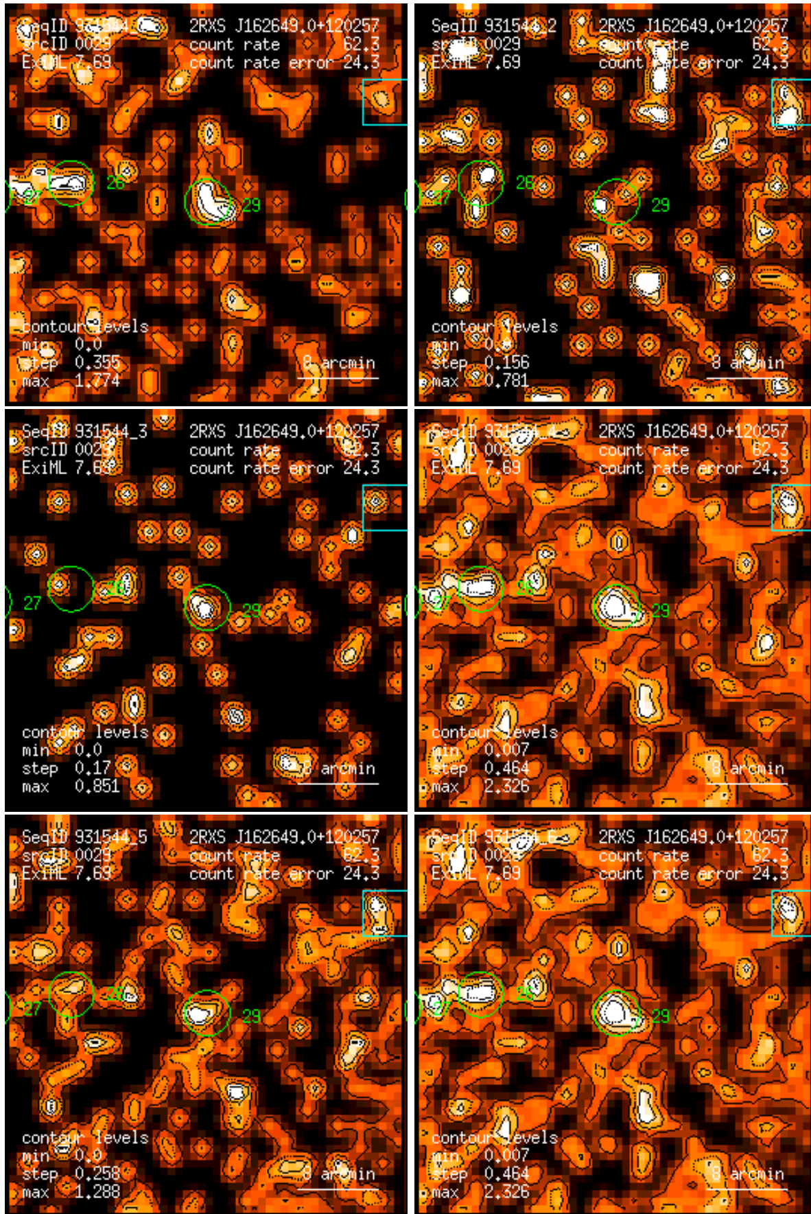
Figure 29: RASS 931544: detection 0029: band rate images, Gaussian filter: (1) PSPC channels 11 – 41, (2) 52 – 90, (3) 91 – 201, (4) 11 – 235, (5) 52 – 201, (6) 11 – 201. Broad band rates in counts/ks. Band rate contour levels in counts/ks/arcmin 2 .
