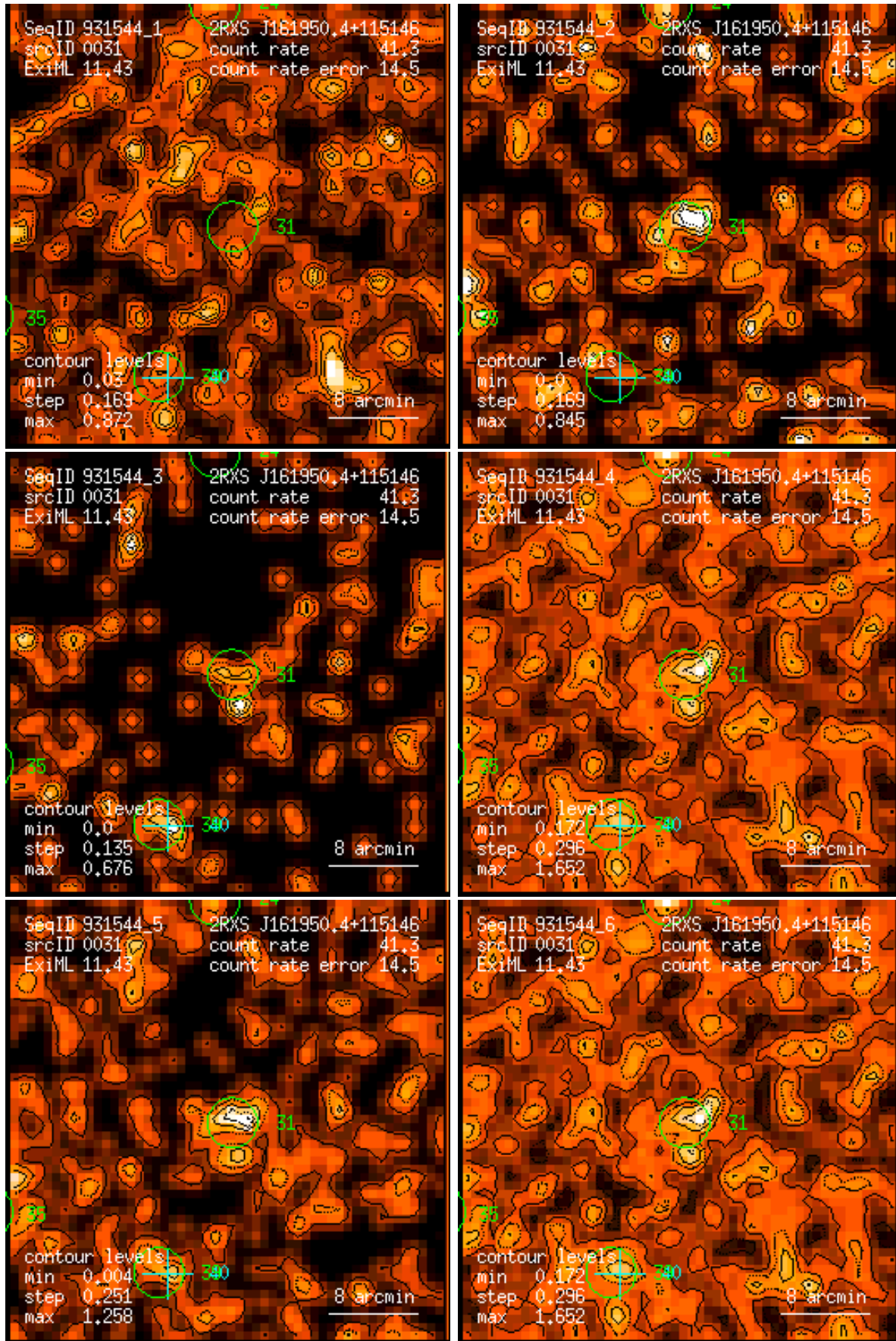
Figure 31: RASS 931544: detection 0031: band rate images, Gaussian filter: (1) PSPC channels 11 – 41, (2) 52 – 90, (3) 91 – 201, (4) 11 – 235, (5) 52 – 201, (6) 11 – 201. Broad band rates in counts/ks. Band rate contour levels in counts/ks/arcmin 2 .
