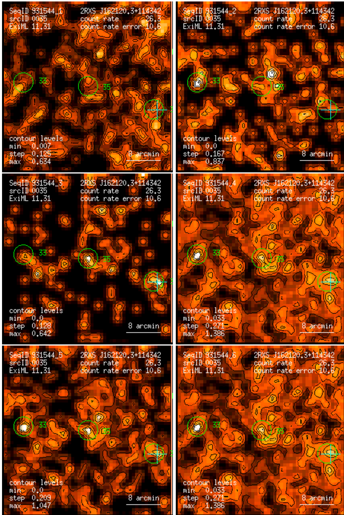
Figure 35: RASS 931544: detection 0035: band rate images, Gaussian filter: (1) PSPC channels 11 – 41, (2) 52 – 90, (3) 91 – 201, (4) 11 – 235, (5) 52 – 201, (6) 11 – 201. Broad band rates in counts/ks. Band rate contour levels in counts/ks/arcmin 2 .
