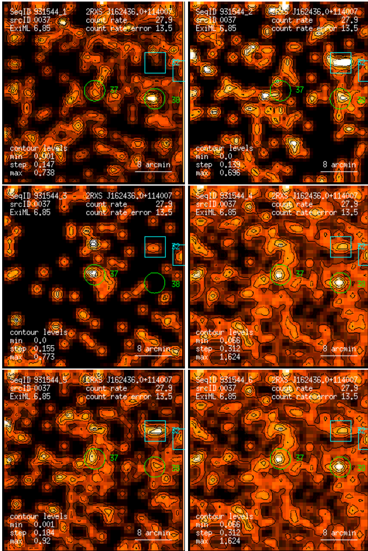
Figure 37: RASS 931544: detection 0037: band rate images, Gaussian filter: (1) PSPC channels 11 – 41, (2) 52 – 90, (3) 91 – 201, (4) 11 – 235, (5) 52 – 201, (6) 11 – 201. Broad band rates in counts/ks. Band rate contour levels in counts/ks/arcmin 2 .
