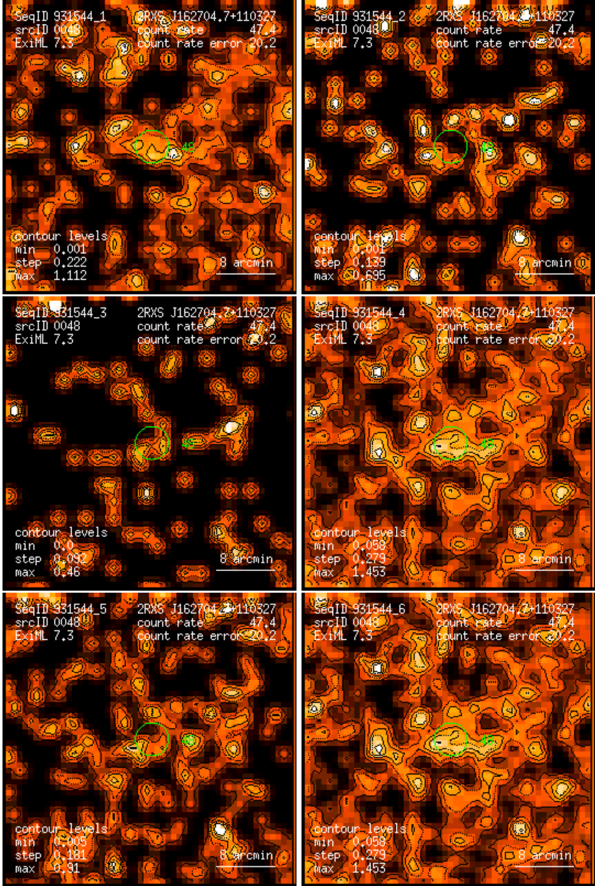
Figure 48: RASS 931544: detection 0048: band rate images, Gaussian filter: (1) PSPC channels 11 – 41, (2) 52 – 90, (3) 91 – 201, (4) 11 – 235, (5) 52 – 201, (6) 11 – 201. Broad band rates in counts/ks. Band rate contour levels in counts/ks/arcmin 2 .
