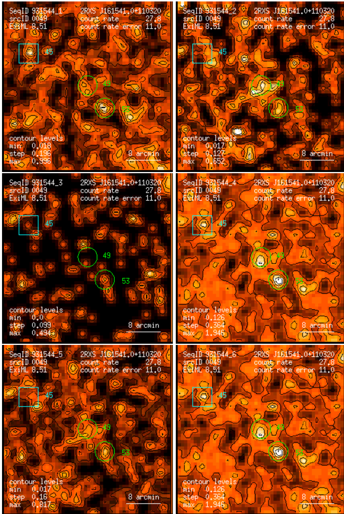
Figure 49: RASS 931544: detection 0049: band rate images, Gaussian filter: (1) PSPC channels 11 – 41, (2) 52 – 90, (3) 91 – 201, (4) 11 – 235, (5) 52 – 201, (6) 11 – 201. Broad band rates in counts/ks. Band rate contour levels in counts/ks/arcmin 2 .
