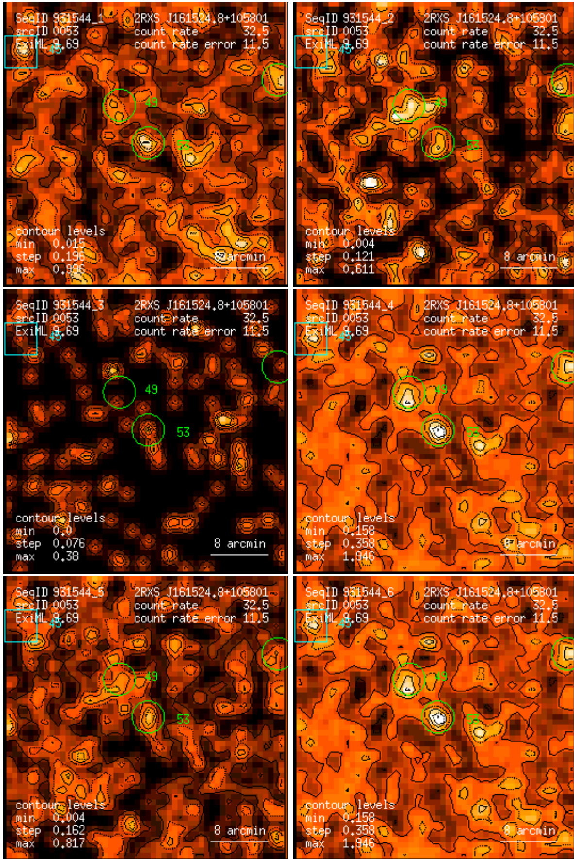
Figure 53: RASS 931544: detection 0053: band rate images, Gaussian filter: (1) PSPC channels 11 – 41, (2) 52 – 90, (3) 91 – 201, (4) 11 – 235, (5) 52 – 201, (6) 11 – 201. Broad band rates in counts/ks. Band rate contour levels in counts/ks/arcmin 2 .
