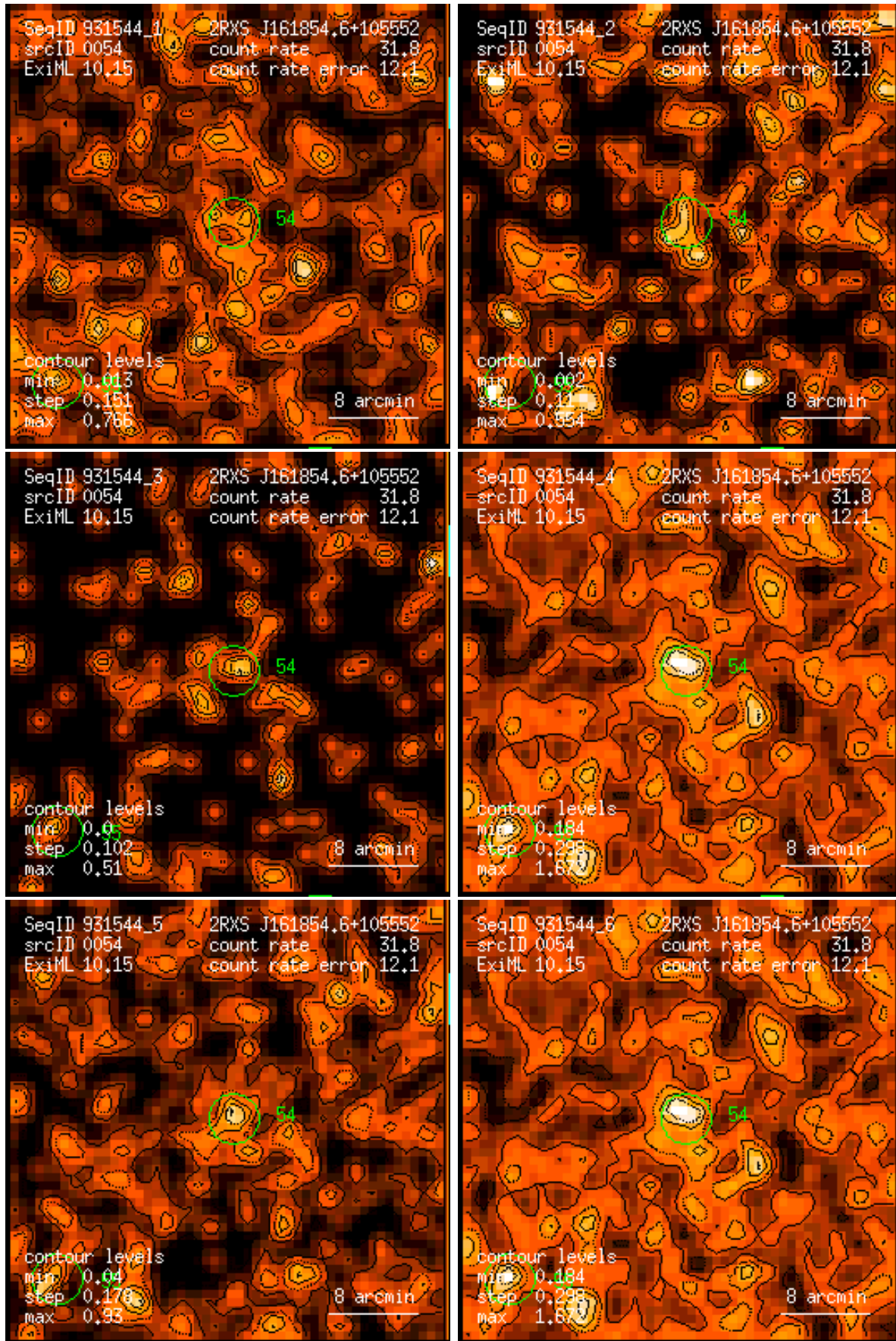
Figure 54: RASS 931544: detection 0054: band rate images, Gaussian filter: (1) PSPC channels 11 – 41, (2) 52 – 90, (3) 91 – 201, (4) 11 – 235, (5) 52 – 201, (6) 11 – 201. Broad band rates in counts/ks. Band rate contour levels in counts/ks/arcmin 2 .
