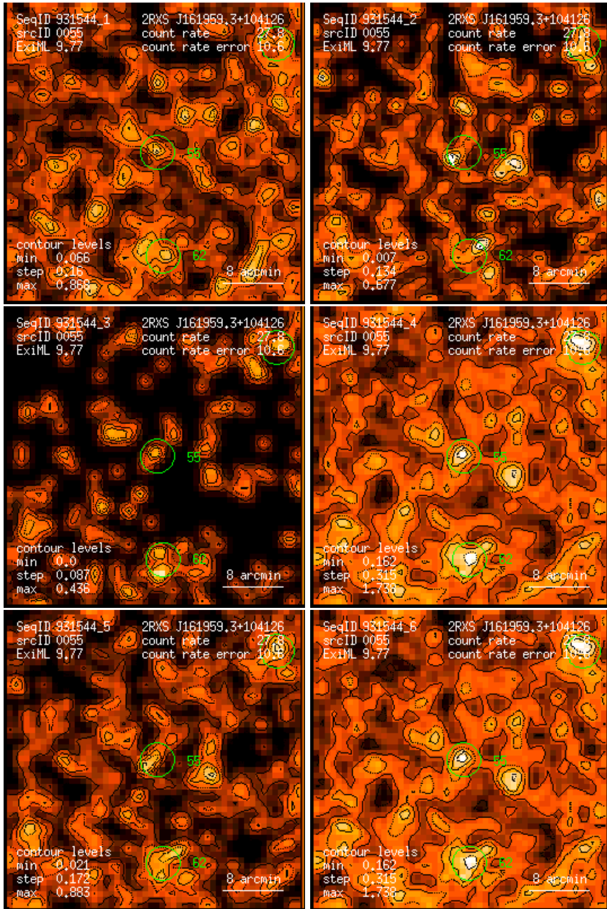
Figure 55: RASS 931544: detection 0055: band rate images, Gaussian filter: (1) PSPC channels 11 – 41, (2) 52 – 90, (3) 91 – 201, (4) 11 – 235, (5) 52 – 201, (6) 11 – 201. Broad band rates in counts/ks. Band rate contour levels in counts/ks/arcmin 2 .
