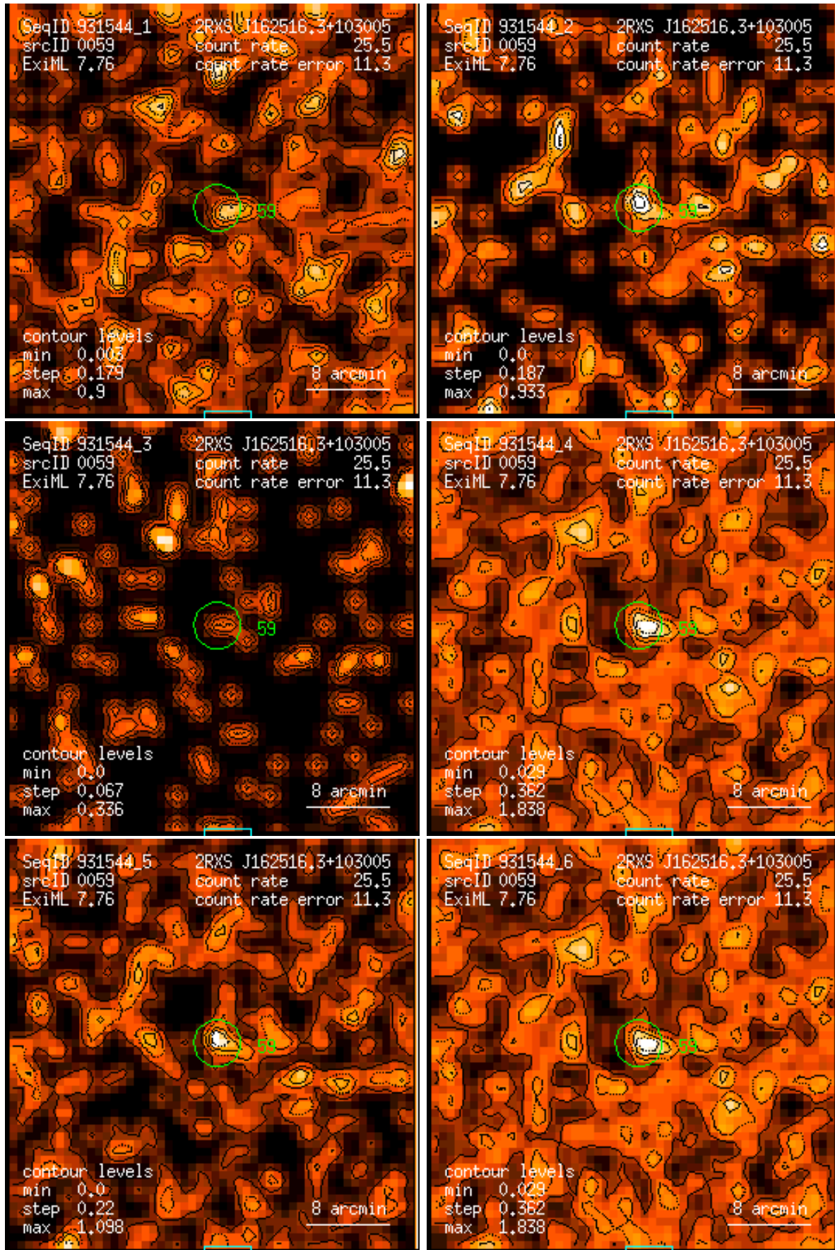
Figure 59: RASS 931544: detection 0059: band rate images, Gaussian filter: (1) PSPC channels 11 – 41, (2) 52 – 90, (3) 91 – 201, (4) 11 – 235, (5) 52 – 201, (6) 11 – 201. Broad band rates in counts/ks. Band rate contour levels in counts/ks/arcmin 2 .
