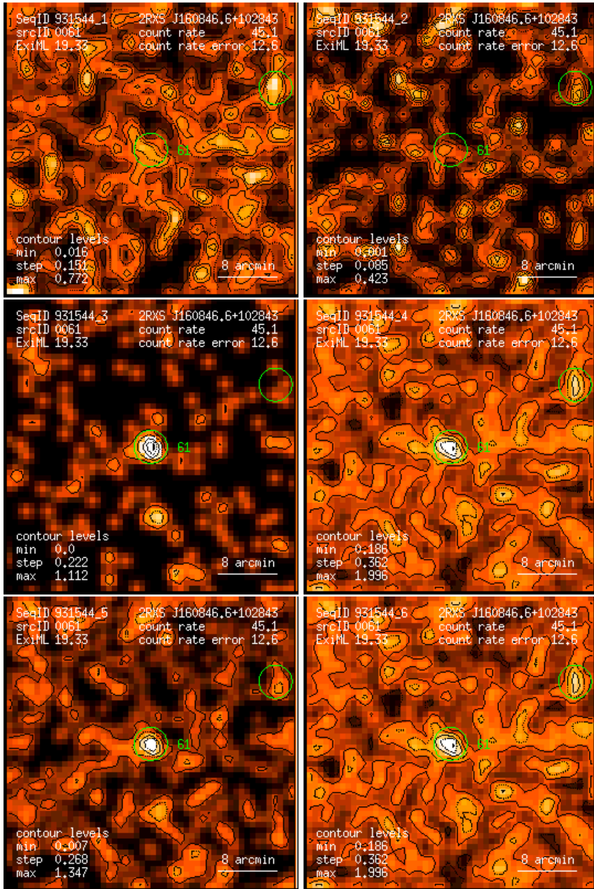
Figure 61: RASS 931544: detection 0061: band rate images, Gaussian filter: (1) PSPC channels 11 – 41, (2) 52 – 90, (3) 91 – 201, (4) 11 – 235, (5) 52 – 201, (6) 11 – 201. Broad band rates in counts/ks. Band rate contour levels in counts/ks/arcmin 2 .
