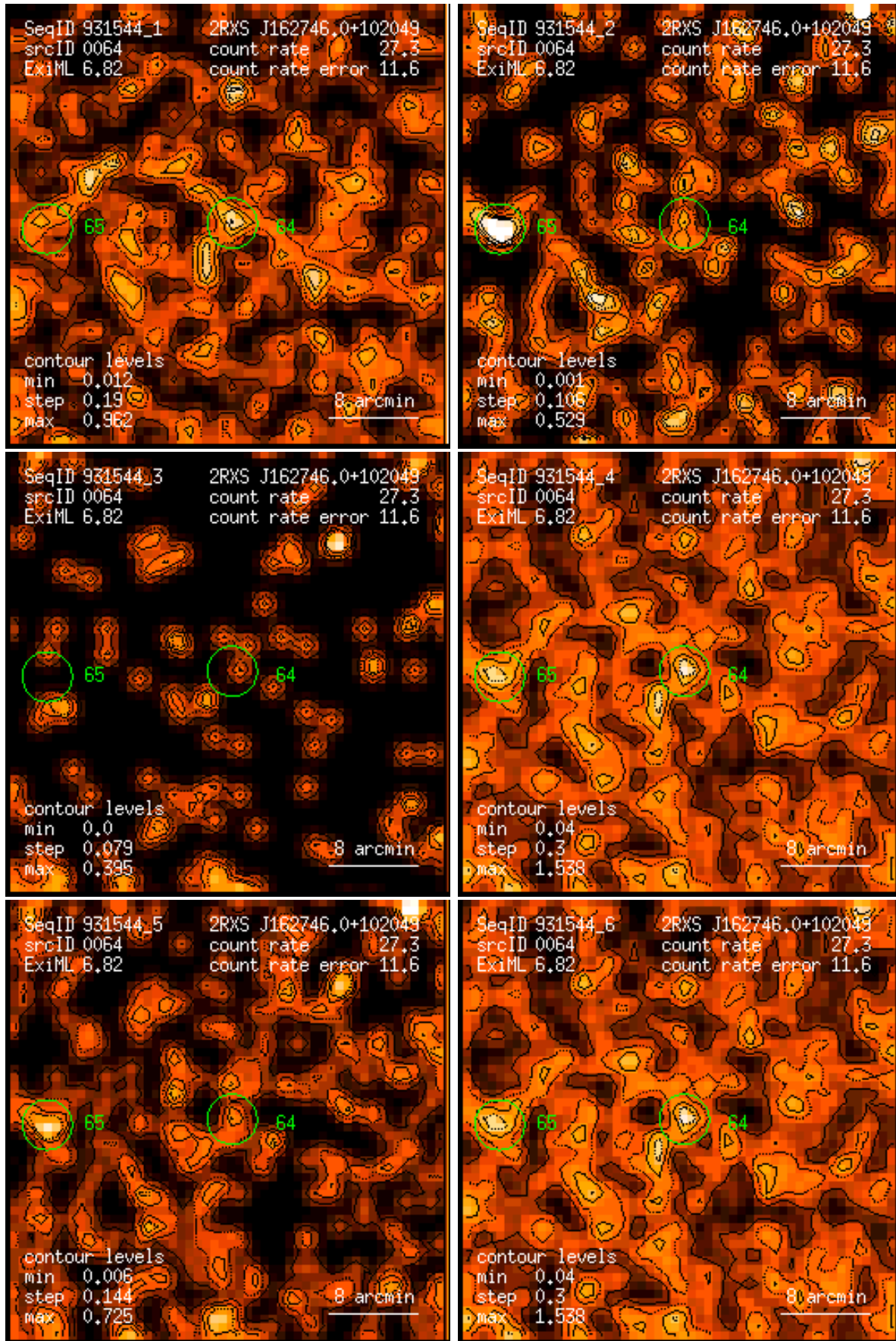
Figure 64: RASS 931544: detection 0064: band rate images, Gaussian filter: (1) PSPC channels 11 – 41, (2) 52 – 90, (3) 91 – 201, (4) 11 – 235, (5) 52 – 201, (6) 11 – 201. Broad band rates in counts/ks. Band rate contour levels in counts/ks/arcmin 2 .
