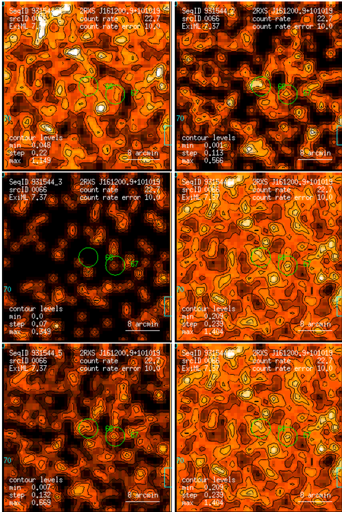
Figure 66: RASS 931544: detection 0066: band rate images, Gaussian filter: (1) PSPC channels 11 – 41, (2) 52 – 90, (3) 91 – 201, (4) 11 – 235, (5) 52 – 201, (6) 11 – 201. Broad band rates in counts/ks. Band rate contour levels in counts/ks/arcmin 2 .
