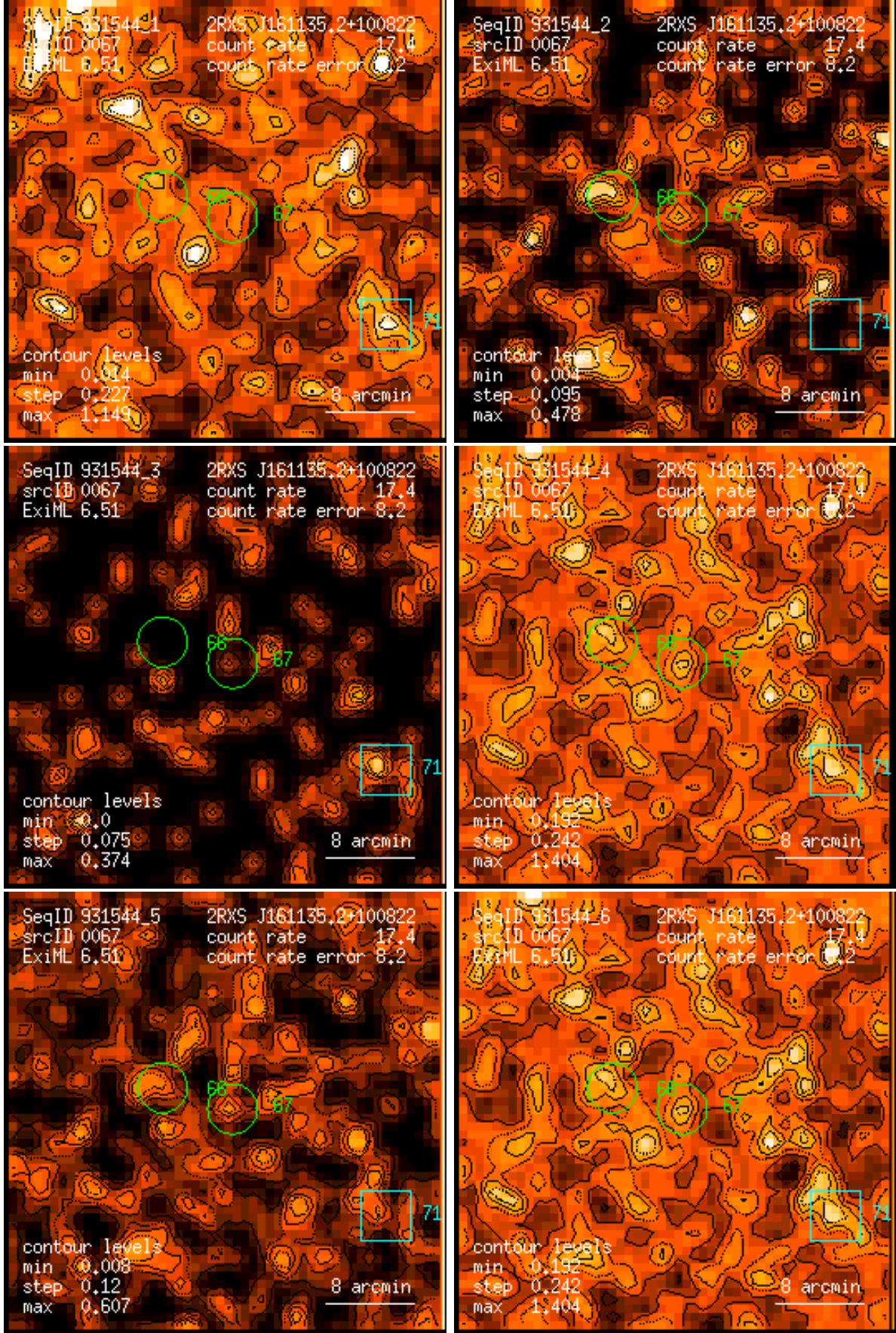
Figure 67: RASS 931544: detection 0067: band rate images, Gaussian filter: (1) PSPC channels 11 – 41, (2) 52 – 90, (3) 91 – 201, (4) 11 – 235, (5) 52 – 201, (6) 11 – 201. Broad band rates in counts/ks. Band rate contour levels in counts/ks/arcmin 2 .
