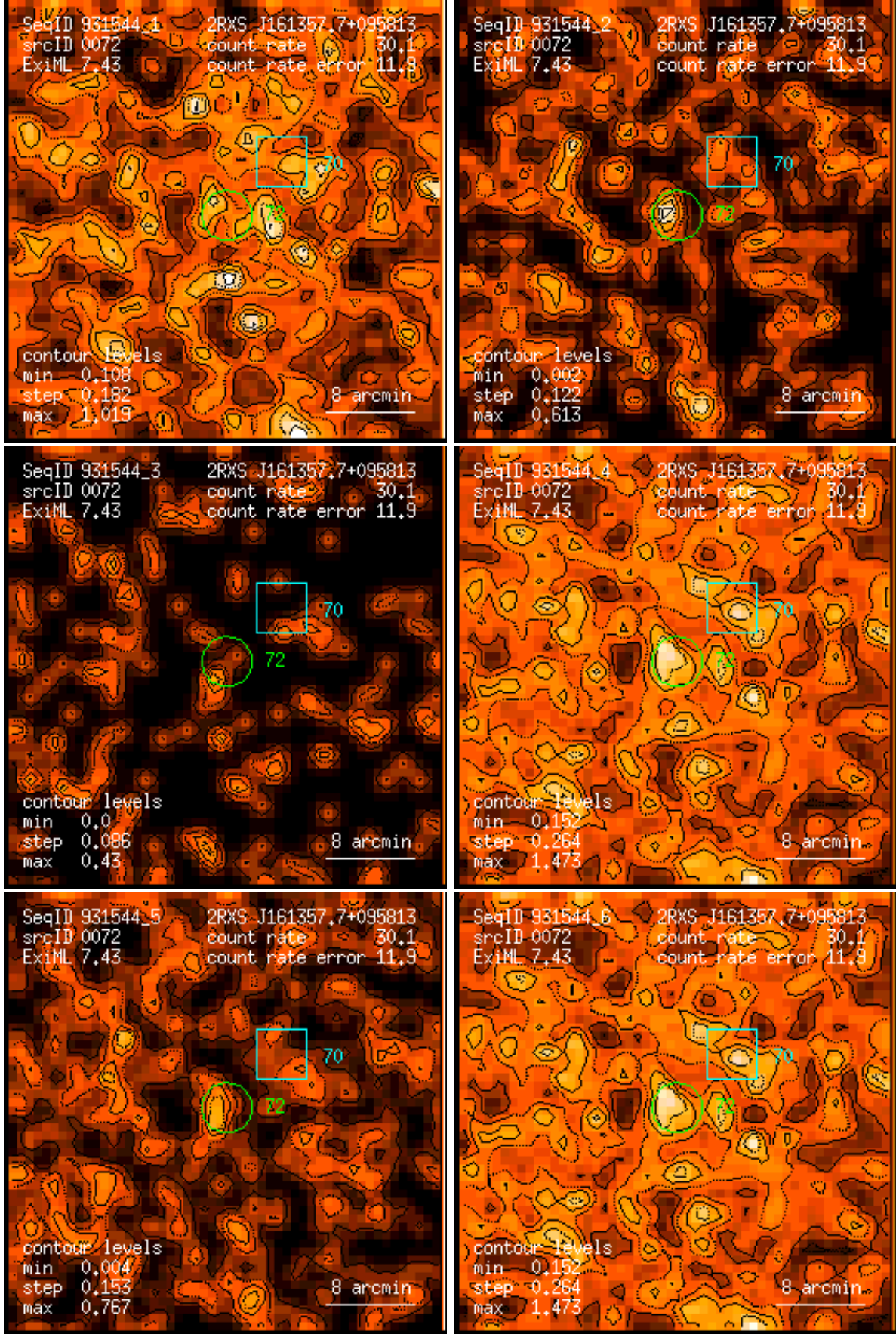
Figure 72: RASS 931544: detection 0072: band rate images, Gaussian filter: (1) PSPC channels 11 – 41, (2) 52 – 90, (3) 91 – 201, (4) 11 – 235, (5) 52 – 201, (6) 11 – 201. Broad band rates in counts/ks. Band rate contour levels in counts/ks/arcmin 2 .
