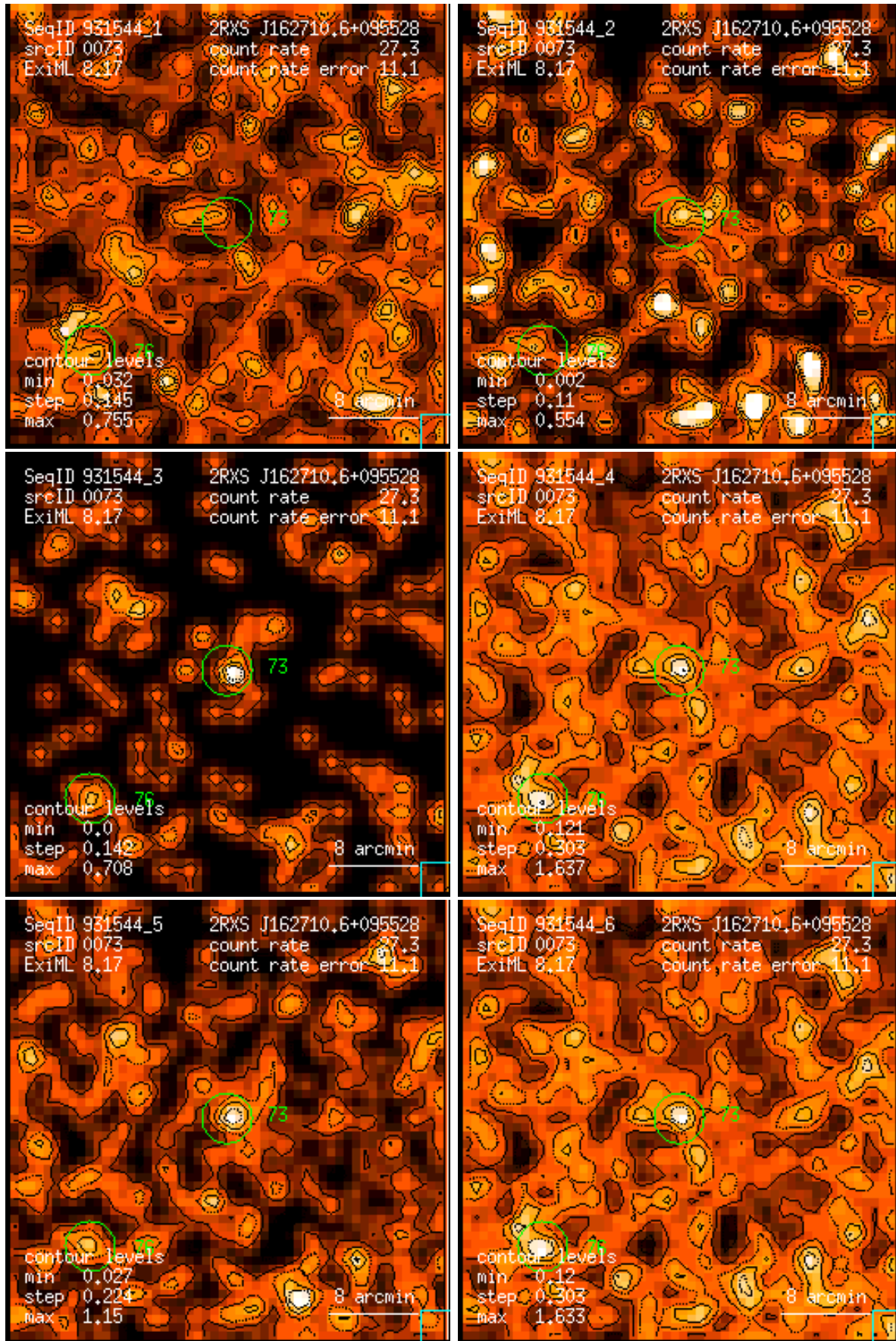
Figure 73: RASS 931544: detection 0073: band rate images, Gaussian filter: (1) PSPC channels 11 – 41, (2) 52 – 90, (3) 91 – 201, (4) 11 – 235, (5) 52 – 201, (6) 11 – 201. Broad band rates in counts/ks. Band rate contour levels in counts/ks/arcmin 2 .
